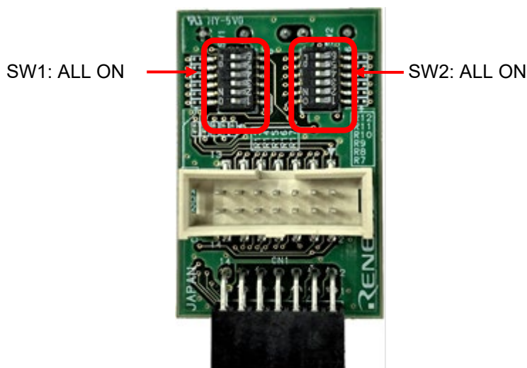
Synchronous adapter for the E2 emulator (RTE0T00020KCAA1000J)
