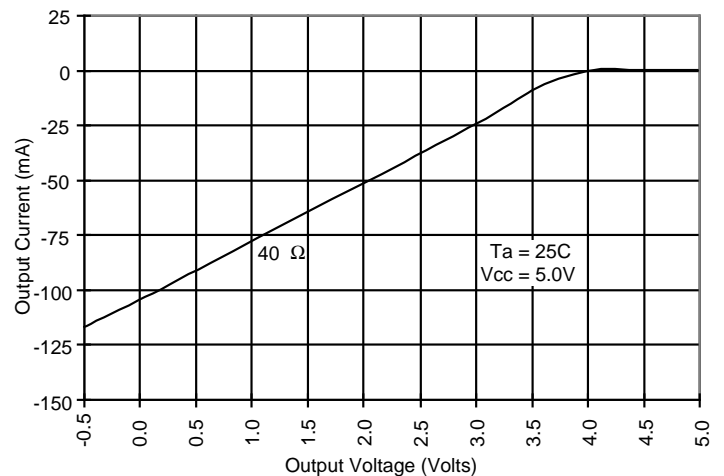
Figure 13, BD-Lite Voh Characteristics
