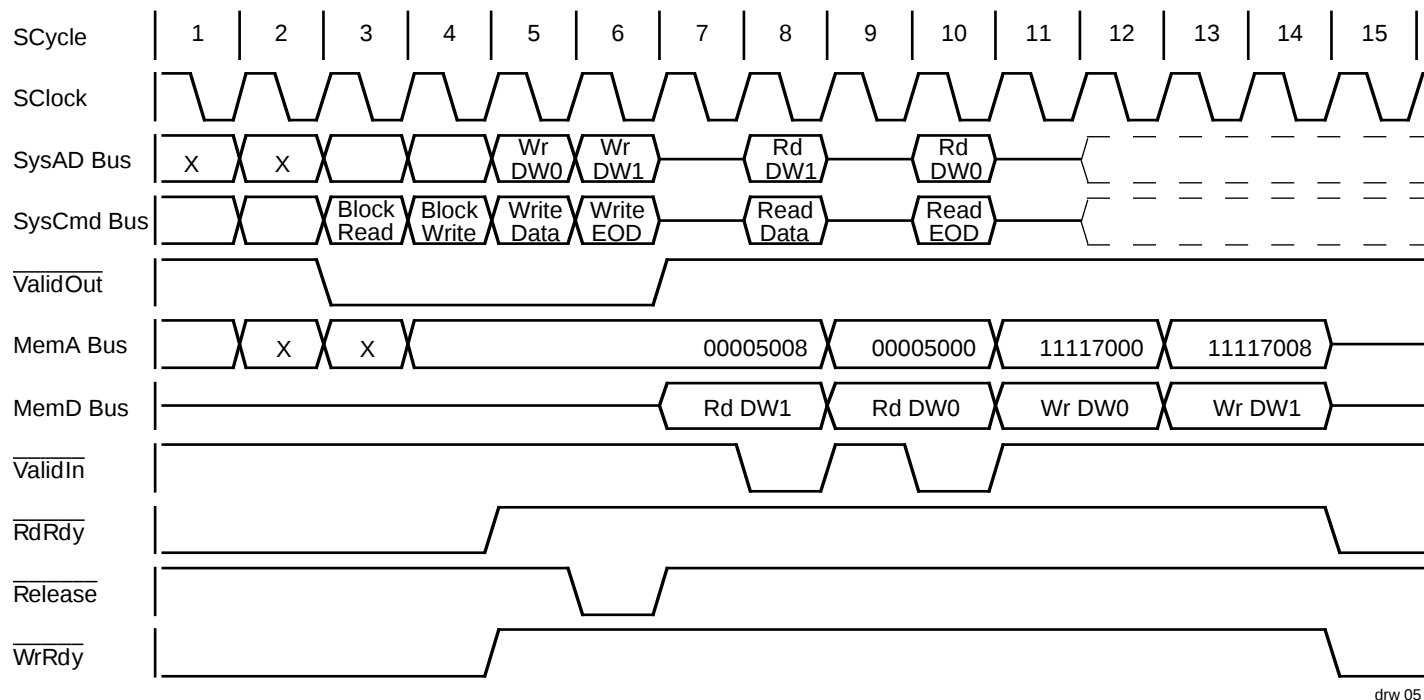
Figure 5. Secondary Cache Overlap Timing
