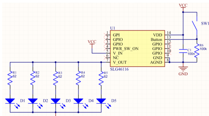
Figure 4. Bike LED tail light typical application circuit
