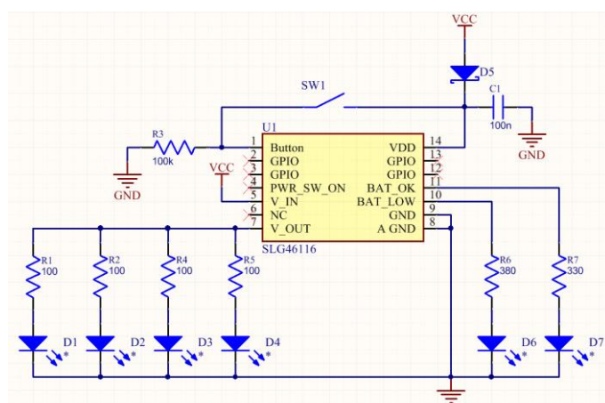
Figure 3. Bike LED headlight typical application circuit
