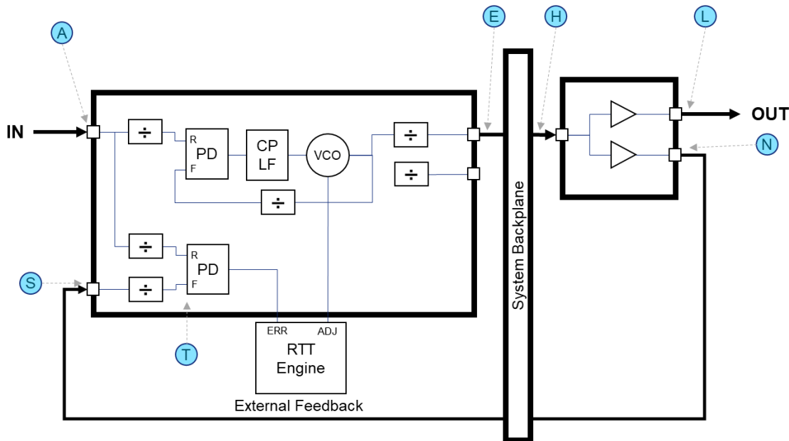
Figure 4. A Simplified Illustration of Round-Trip Time (RTT)
