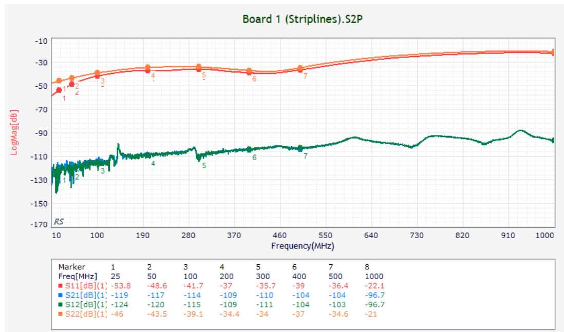
Figure 6. Board 1 (Striplines)
