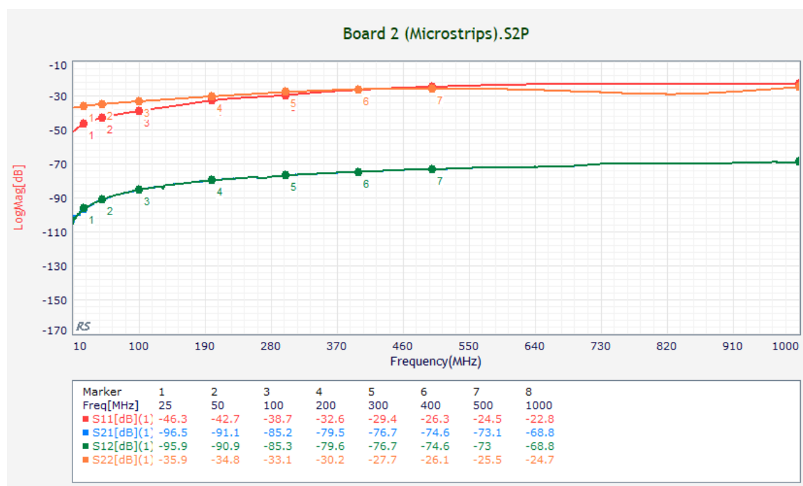
Figure 7. Board 2 (Microstrips)
