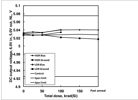
Figure 26: ISL75051SEH DC output voltage, 5.0V output, 6.0V input, no load, as a function of biased and grounded high and low dose rate irradiation and subsequent high temperature accelerated post-high dose rate aging at 100°C. The dose rate was 80 rad(Si)/s. Sample size was 6 for the high dose rate cells and 4 for the low dose rate cells, and three control units were used for the high dose rate test. The specification limits are 4.9250V – 5.0750V.
