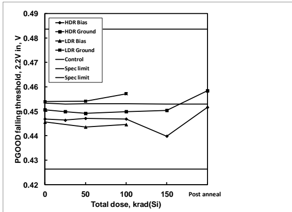
Figure 47: ISL75051SEH PGOOD falling threshold, 2.2V in, as a function of biased and grounded high and low dose rate irradiation and subsequent high temperature accelerated post-high dose rate aging at 100°C. The dose rate was 80 rad(Si)/s. Sample size was 6 for the high dose rate cells and 4 for the low dose rate cells, and three control units were used for the high dose rate test. The specification limits are 0.4420V to 0.4992V.
