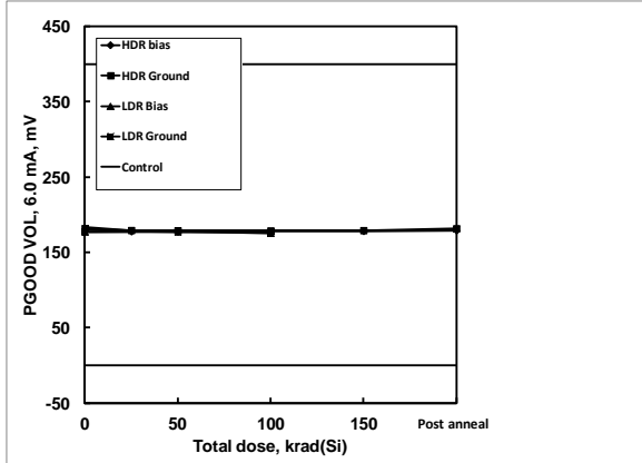
Figure 42: ISL75051SEH PGOOD output LOW voltage, 6mA, as a function of biased and grounded high and low dose rate irradiation and subsequent high temperature accelerated post-high dose rate aging at 100°C. The dose rate was 80 rad(Si)/s. Sample size was 6 for the high dose rate cells and 4 for the low dose rate cells, and three control units were used for the high dose rate test. The specification limits are 0mV to 400.0mV.
