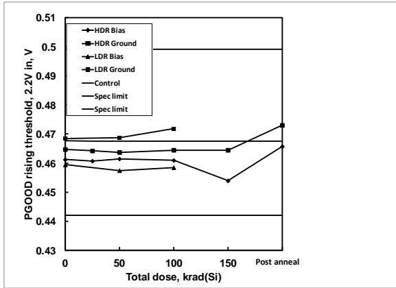
Figure 46: ISL75051SEH PGOOD rising threshold, 2.2V in, as a function of biased and grounded high and low dose rate irradiation and subsequent high temperature accelerated post-high dose rate aging at 100°C. The dose rate was 80 rad(Si)/s. Sample size was 6 for the high dose rate cells and 4 for the low dose rate cells, and three control units were used for the high dose rate test. The specification limits are 0.4264V to 0.4836V.
