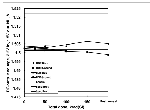
Figure 16: ISL75051SEH DC output voltage, 1.5V output, 2.2V input, no load, as a function of biased and grounded high and low dose rate irradiation and subsequent high temperature accelerated post-high dose rate aging at 100°C. The dose rate was 80 rad(Si)/s. Sample size was 6 for the high dose rate cells and 4 for the low dose rate cells, and three control units were used for the high dose rate test. The specification limits are 1.4780V – 1.5220V.
