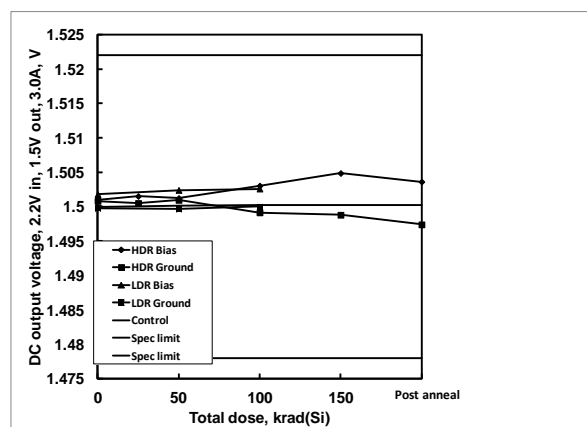
Figure 17: ISL75051SEH DC output voltage, 1.5V output, 2.2V input, 3A load, as a function of biased and grounded high and low dose rate irradiation and subsequent high temperature accelerated post-high dose rate aging at 100°C. The dose rate was 80 rad(Si)/s. Sample size was 6 for the high dose rate cells and 4 for the low dose rate cells, and three control units were used for the high dose rate test. The specification limits are 1.4780V – 1.5220V.
