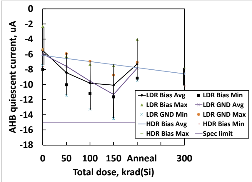
Fig. 6: HS-4080AEH A high side bootstrap supply quiescent current as a function of total dose irradiation at low dose rate for the biased (per Figure 1) and unbiased (all pins grounded) cases and at high dose rate for the biased case. The dose rate was 0.01 rad(Si)/s for low dose rate irradiation and 68 rad(Si)/s for high dose rate irradiation. The low dose rate irradiations were followed by a biased anneal at 100°C for 168 hours. Sample sizes were 10 at low dose rate under bias, 10 at low dose rate with all pins grounded and 20 samples at high dose rate under bias. The SMD post-irradiation specification limit is -15.0uA maximum. (127)
