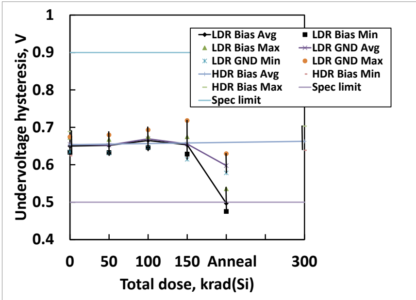
Fig. 27: HS-4080AEH undervoltage hysteresis voltage as a function of total dose irradiation at low dose rate for the biased (per Figure 1) and unbiased (all pins grounded) cases and at high dose rate for the biased case. The dose rate was 0.01 rad(Si)/s for low dose rate irradiation and 68 rad(Si)/s for high dose rate irradiation. The low dose rate irradiations were followed by a biased anneal at 100°C for 168 hours. Sample sizes were 10 at low dose rate under bias, 10 at low dose rate with all pins grounded and 20 samples at high dose rate under bias. The SMD post-irradiation specification limits are 0.5V to 0.9V. (152)
