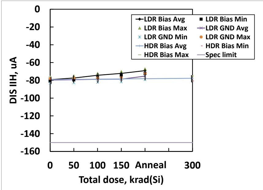
Fig. 20: HS-4080AEH disable (DIS) pin HIGH input current as a function of total dose irradiation at low dose rate for the biased (per Figure 1) and unbiased (all pins grounded) cases and at high dose rate for the biased case. The dose rate was 0.01 rad(Si)/s for low dose rate irradiation and 68 rad(Si)/s for high dose rate irradiation. The low dose rate irradiations were followed by a biased anneal at 100°C for 168 hours. Sample sizes were 10 at low dose rate under bias, 10 at low dose rate with all pins grounded and 20 samples at high dose rate under bias. The SMD post-irradiation specification limit is -150.0uA maximum. (121)
