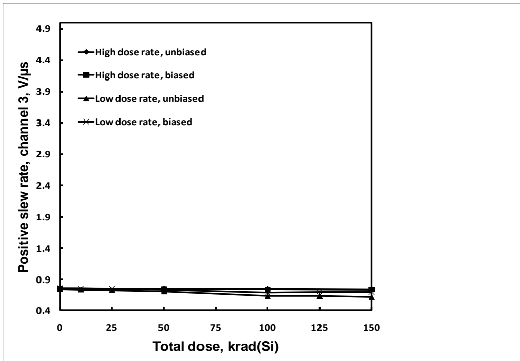
Figure 50: ISL7124SRH positive slew rate, channel 3, as a function of total dose irradiation at low and high dose rate for the unbiased and biased cases. The post-irradiation SMD limit is .4V/\mu s .
