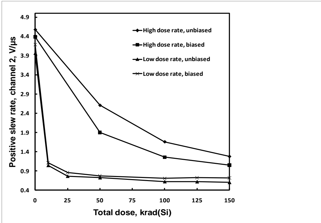
Figure 49: ISL7124SRH positive slew rate, channel 2, as a function of total dose irradiation at low and high dose rate for the unbiased and biased cases. The post-irradiation SMD limit is .4V/\mu s .
