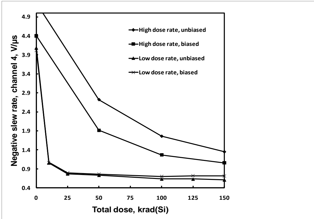
Figure 55: ISL7124SRH negative slew rate, channel 4, as a function of total dose irradiation at low and high dose rate for the unbiased and biased cases. The post-irradiation SMD limit is .4V/\mu s .
