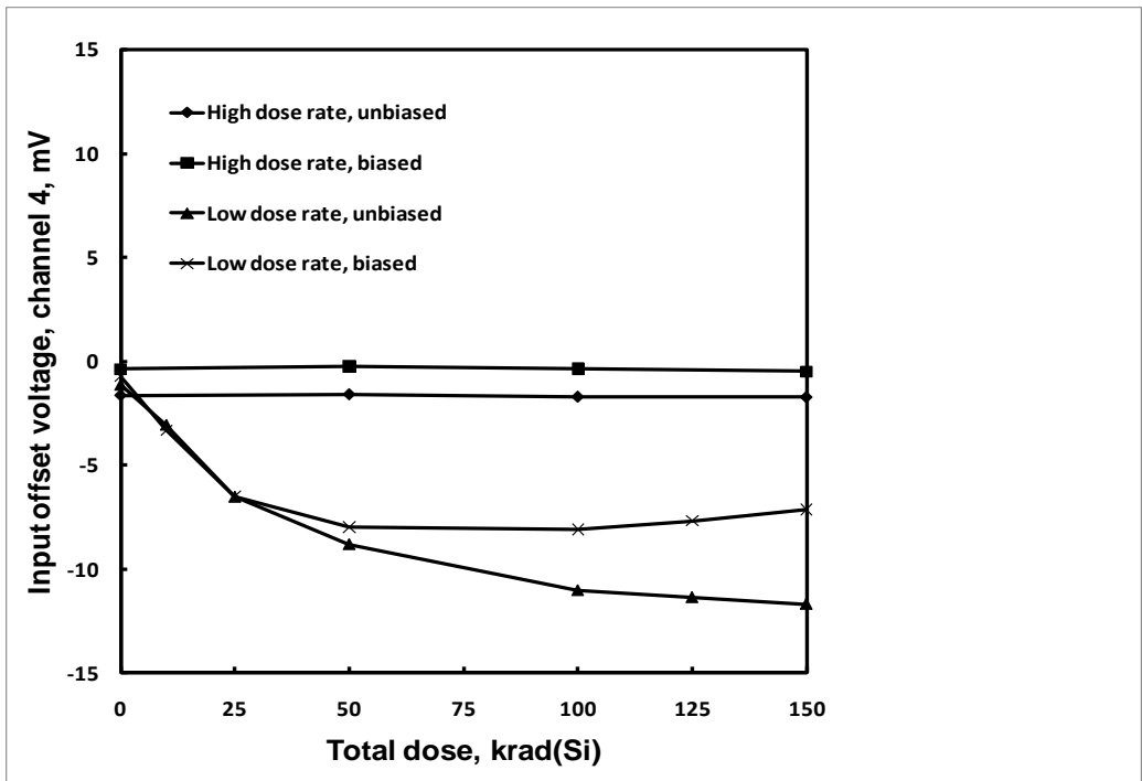
Figure 6: ISL7124SRH input offset voltage, channel 4, as a function of total dose irradiation at low and high dose rate for the unbiased and biased cases. The post-irradiation SMD limits are -10mV to +10mV.
