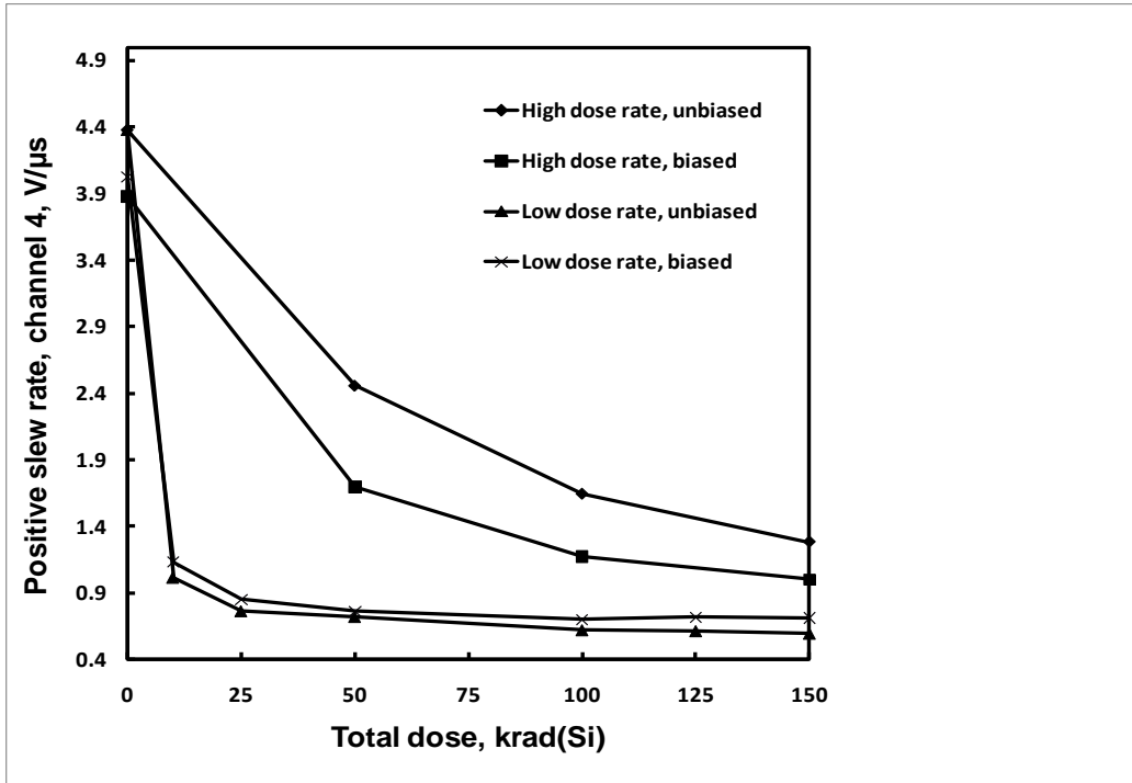
Figure 51: ISL7124SRH positive slew rate, channel 4, as a function of total dose irradiation at low and high dose rate for the unbiased and biased cases. The post-irradiation SMD limit is .4V/\mu s .
