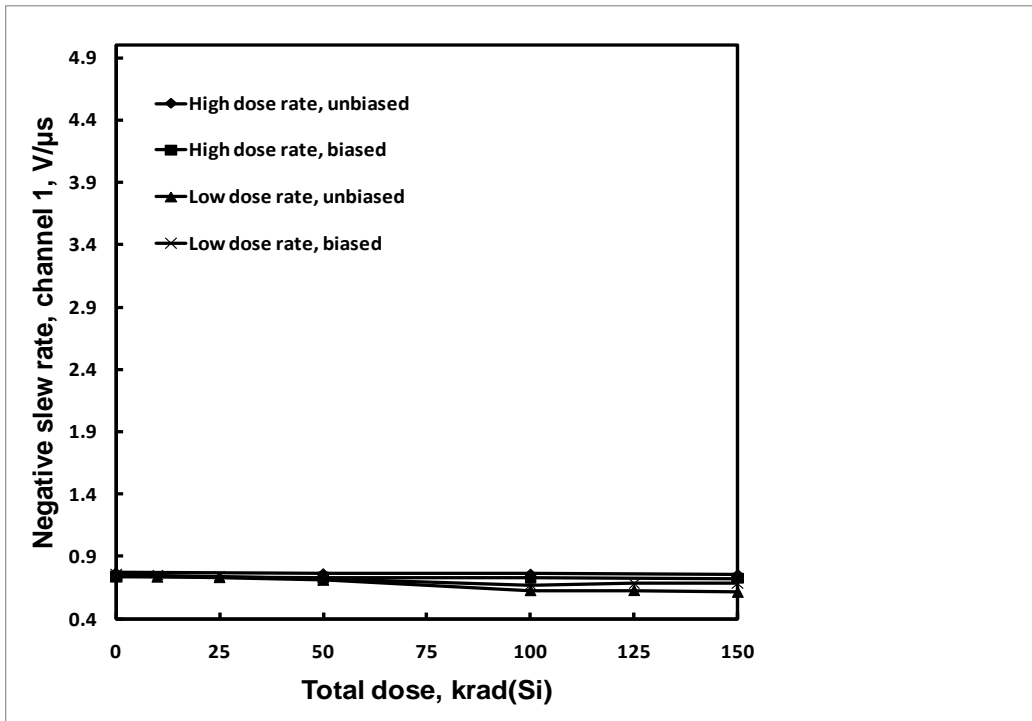
Figure 52: ISL7124SRH negative slew rate, channel 1, as a function of total dose irradiation at low and high dose rate for the unbiased and biased cases. The post-irradiation SMD limit is .4V/\mu s .
