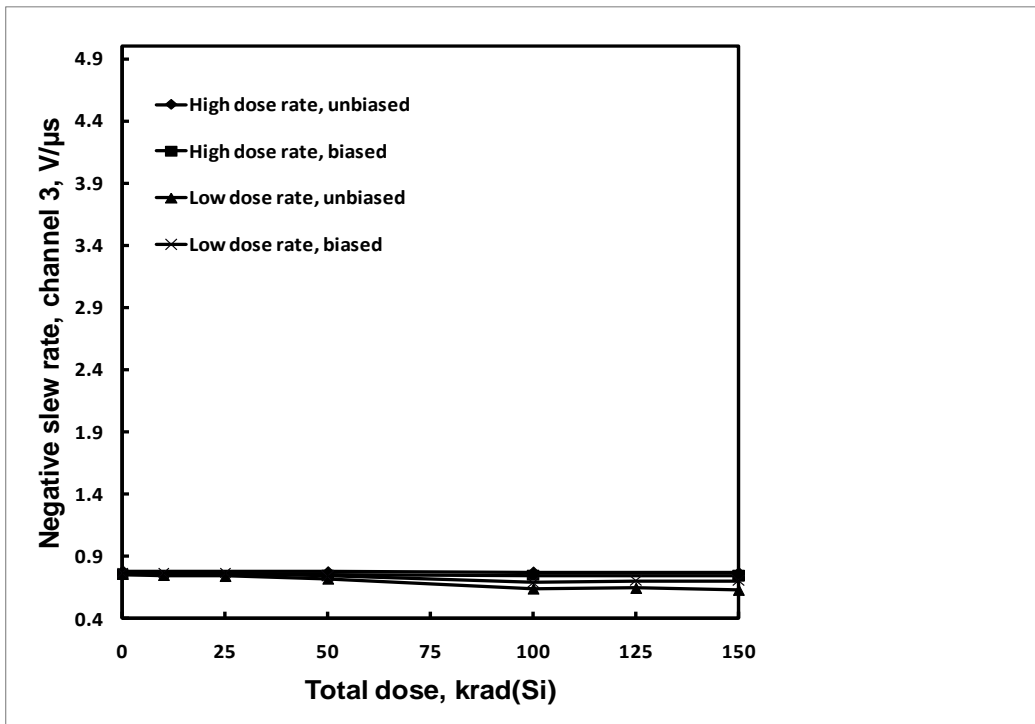
Figure 54: ISL7124SRH negative slew rate, channel 3, as a function of total dose irradiation at low and high dose rate for the unbiased and biased cases. The post-irradiation SMD limit is .4V/\mu s .
