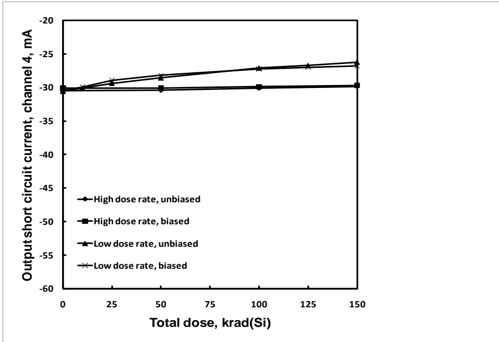
Figure 59: ISL7124SRH output short circuit current, channel 4, as a function of total dose irradiation at low and high dose rate for the unbiased and biased cases. The post-irradiation SMD limit is -60mA maximum.
