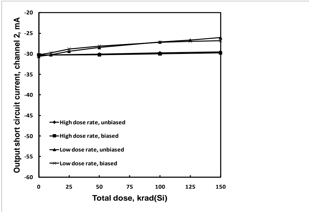
Figure 57: ISL7124SRH output short circuit current, channel 2, as a function of total dose irradiation at low and high dose rate for the unbiased and biased cases. The post-irradiation SMD limit is -60mA maximum.
