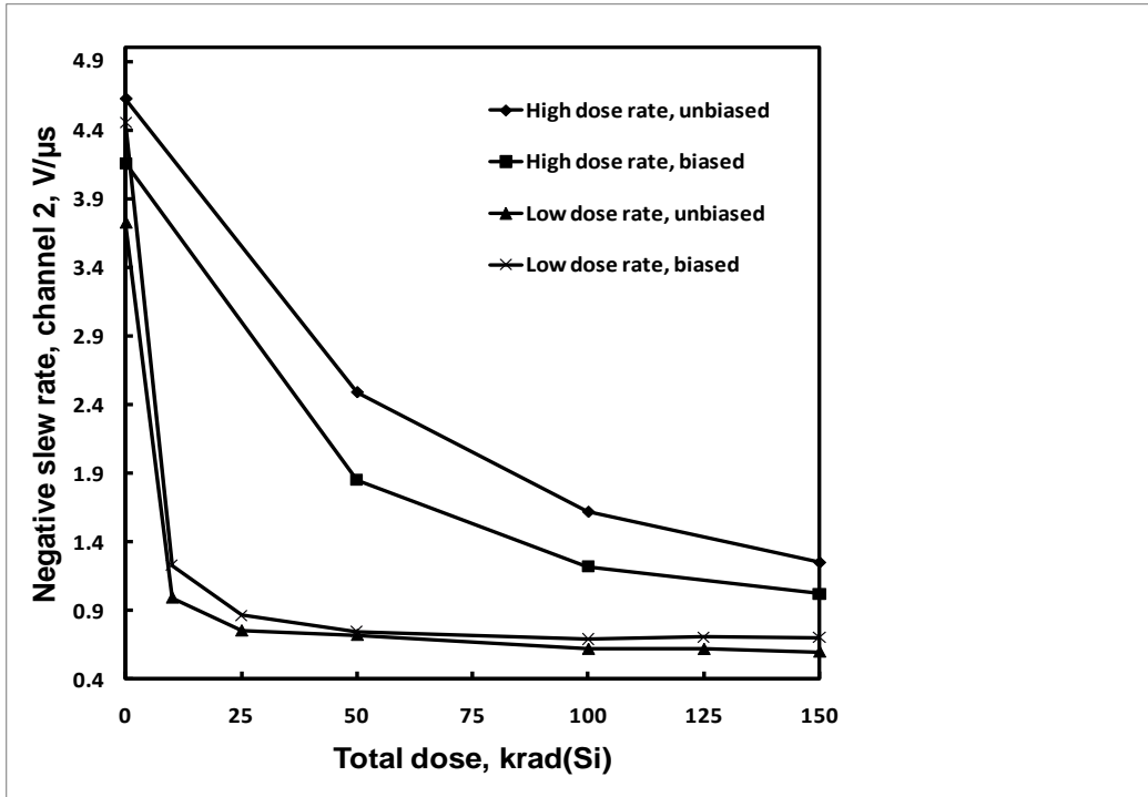
Figure 53: ISL7124SRH negative slew rate, channel 2, as a function of total dose irradiation at low and high dose rate for the unbiased and biased cases. The post-irradiation SMD limit is .4V/\mu s .
