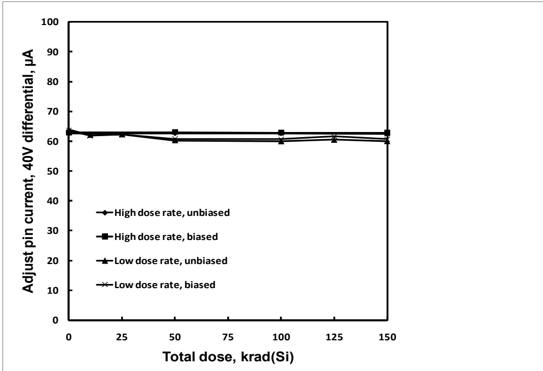
Figure 7: HS-117RH adjust pin current at 40V differential as a function of total dose irradiation at low and high dose rate for the unbiased and biased cases. The post-irradiation SMD limit is 100μA.
