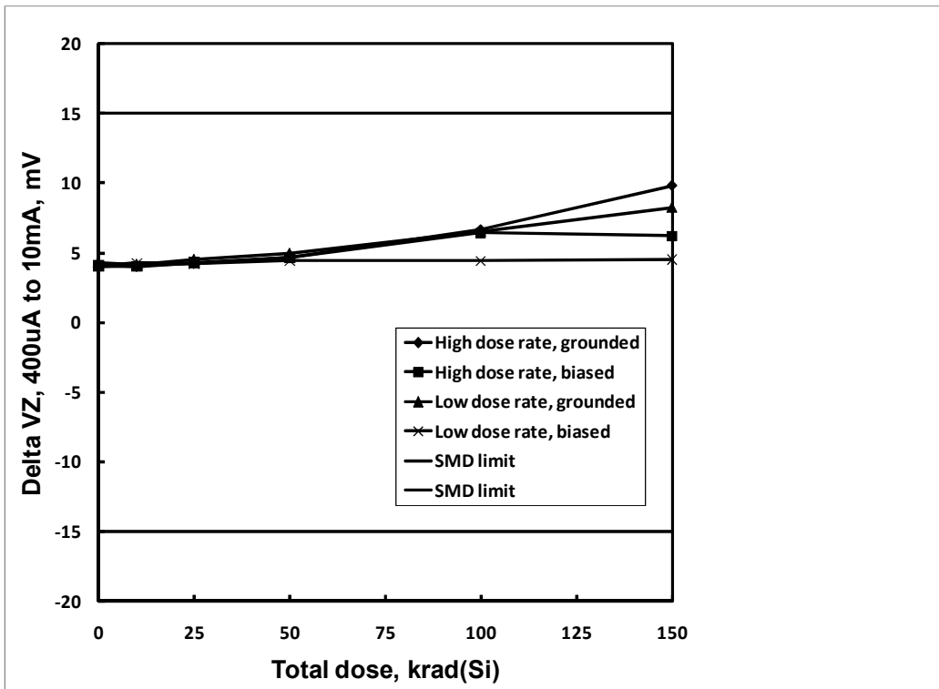
Fig. 5: IS-1009RH total reference voltage variation, 400 \mu A to 10mA output current, as a function of total dose irradiation at low and high dose rate for the unbiased and biased cases. The post-irradiation SMD limits are -15mV to 15mV.
