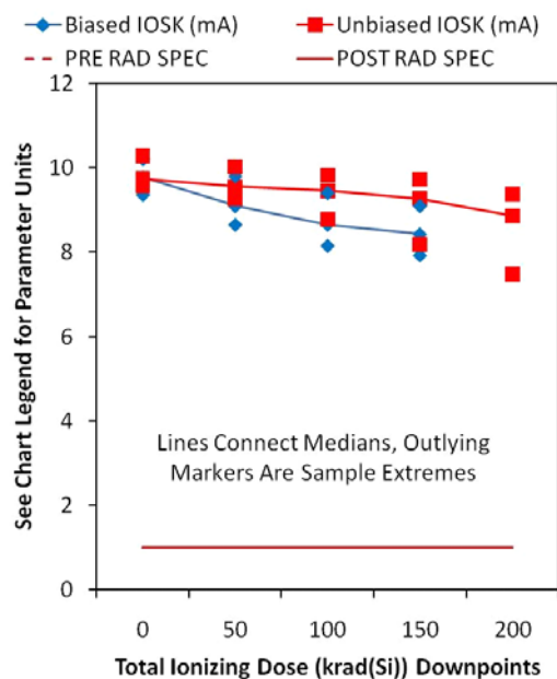
FIGURE 17. ERROR AMPLIFIER OUTPUT SINK CURRENT ( I_{0SK} )
