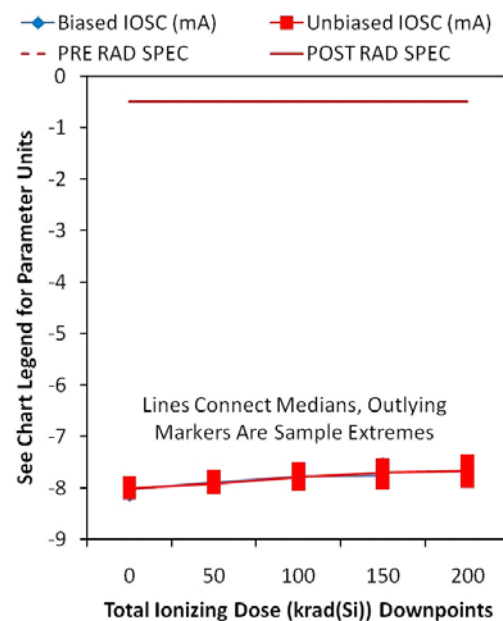
FIGURE 18. ERROR AMPLIFIER OUTPUT SOURCE CURRENT ( I_{0SC} )
