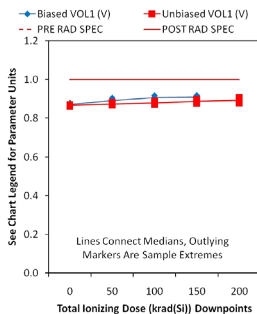
FIGURE 20. ERROR AMPLIFIER OUTPUT LOW VOLTAGE ( V_{0L1} )
