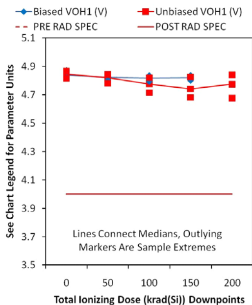
FIGURE 19. ERROR AMPLIFIER OUTPUT HIGH VOLTAGE ( V_{0H1} )
