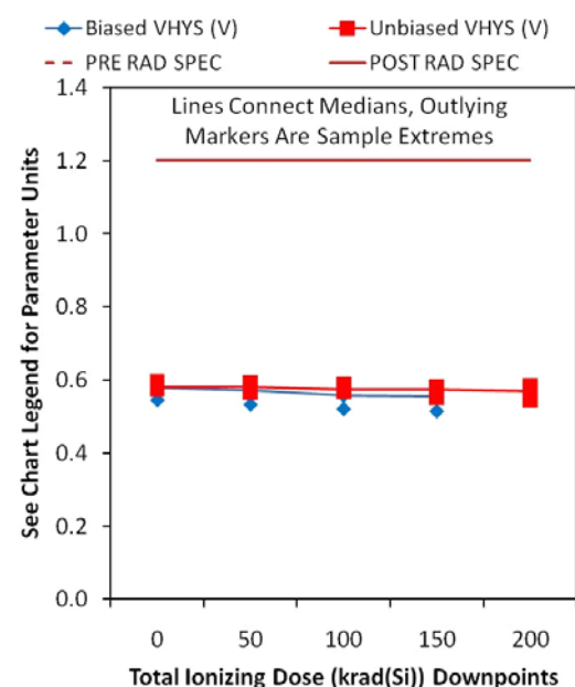
FIGURE 35. UNDERVOLTAGE LOCK-OUT HYSTERESIS VOLTAGE ( V_{HYS} )
