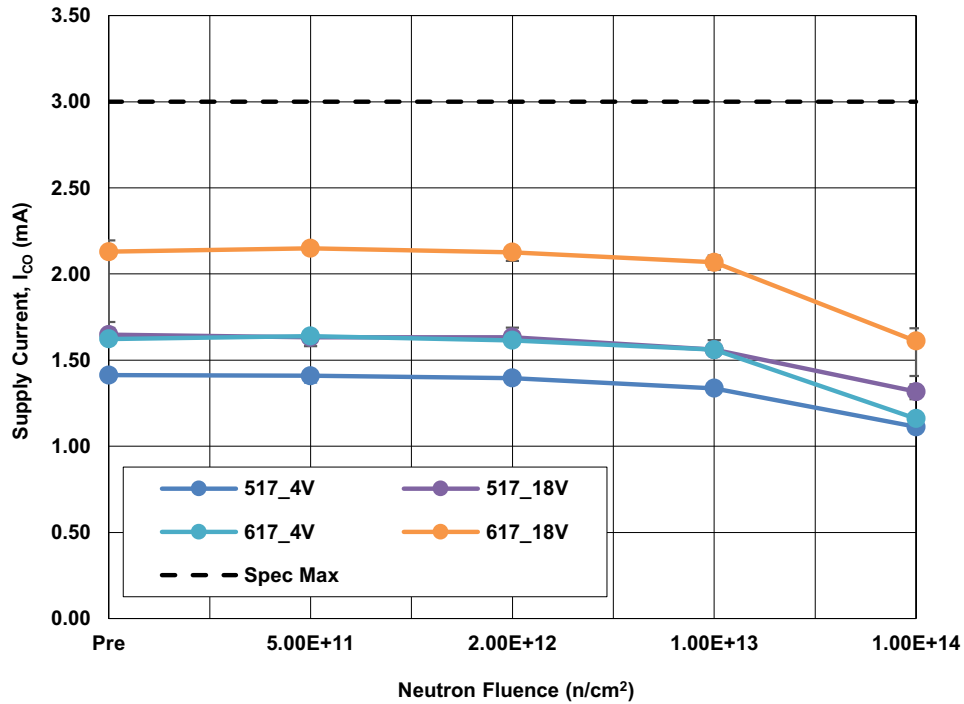
Figure 27. ISL70x17SEH supply current (I CO ) at ±4V and ±18V following irradiation to each level. The error bars represent the minimum and maximum measured values. The SMD limit is 3mA maximum.
