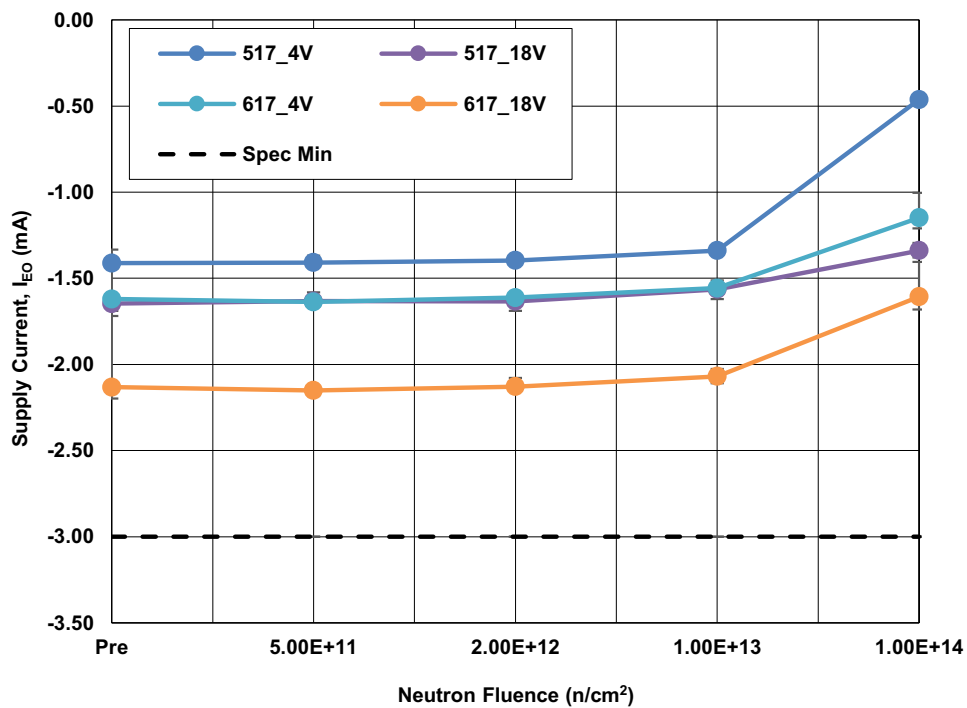
Figure 28. ISL70x17SEH supply current (I EO ) at ±4V and ±18V following irradiation to each level. The error bars represent the minimum and maximum measured values. The SMD limit is -3mA minimum.
