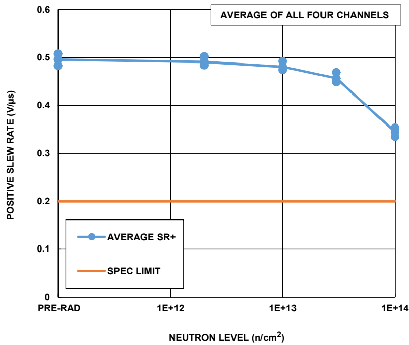
FIGURE 26. ISL70419SEH positive slew rate, average of all four channels, as a function of 1MeV equivalent neutron irradiation at 2 \times 10^{12} \text{ n/cm}^2 , 1 \times 10^{13} \text{ n/cm}^2 , 3 \times 10^{13} \text{ n/cm}^2 , and 1 \times 10^{14} \text{ n/cm}^2 . The plot shows the population median, minimum, and maximum at each downpoint. Sample size for each cell was five. The post-total dose irradiation SMD limit is 0.2 \text{ V}/\mu\text{s} minimum.
