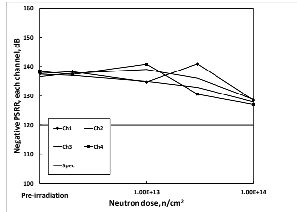
Fig. 8: ISL70417SEH negative power supply rejection ratio (PSRR), +/-15V supplies, each channel, as a function of neutron irradiation. Sample size was 5 for each cell ( 2 \times 10^{12} n/cm 2 , 1 \times 10^{13} n/cm 2 , 3 \times 10^{13} n/cm 2 and 1 \times 10^{14} n/cm 2 ), with two control units. The post-irradiation SMD limit is 120dB minimum.
