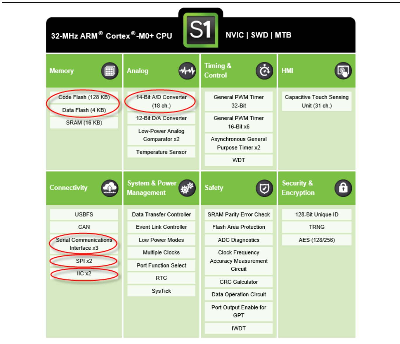
Figure 1. S1 peripherals used by the OoB
