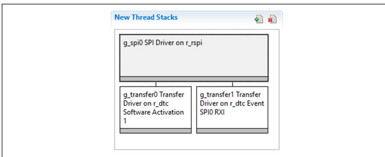
Figure 2. RSPI HAL Module Stack
