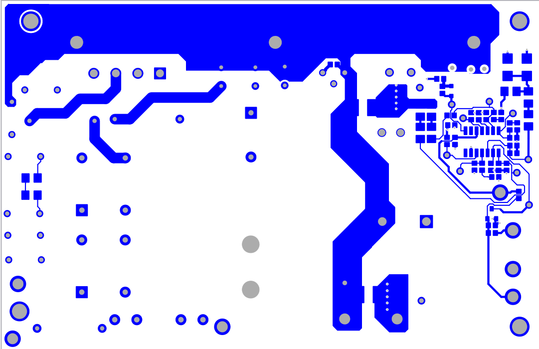
FIGURE 5. TOP LAYER
