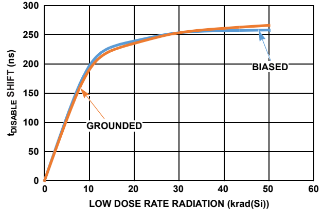
FIGURE 55. t_{DISABLE} SHIFT vs LDR RADIATION
