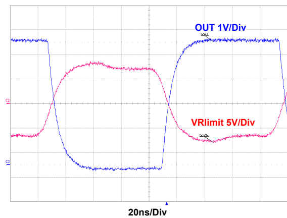
Figure 17. Switching, Coil Current \sim \pm 18mA , C_{BOOST} = 15pF , C_{OUT} = 15pF , V_{DD} = 5V
