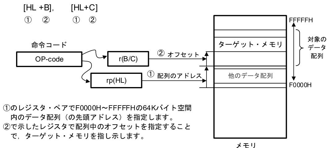
図3-35 [HL+B], [HL+C]の例
