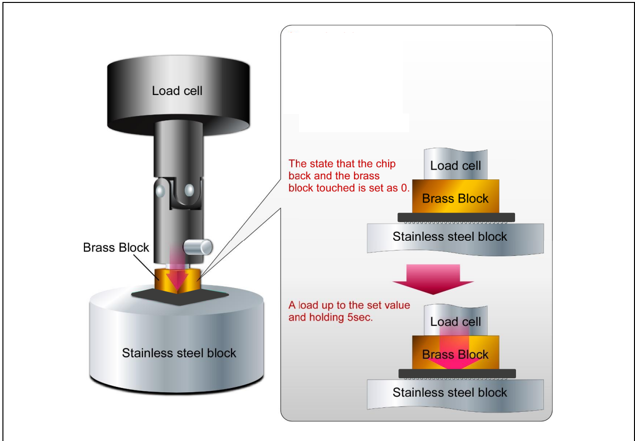
Figure 1.1 Stress testing machine image
