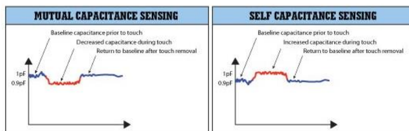
Figure 4: Mutual- and self-capacitance sensing
