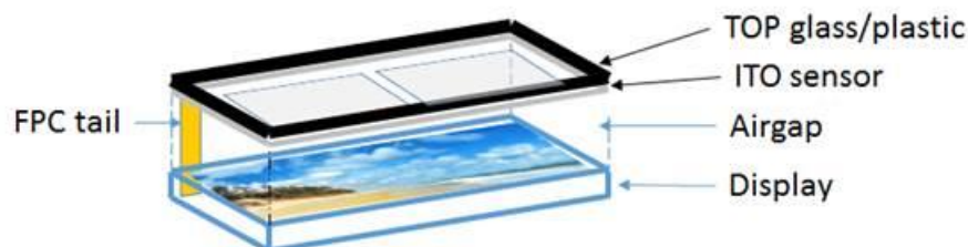
Figure 11: ITO placement underneath the top glass cover
