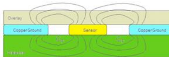
Figure 1: Cross section of a capacitive sensor laid on PCB
