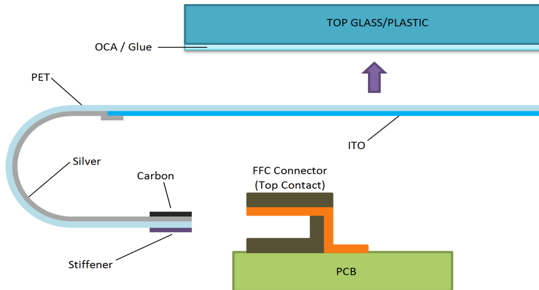
Figure 12: Complete top-level ITO placement on a PCB
