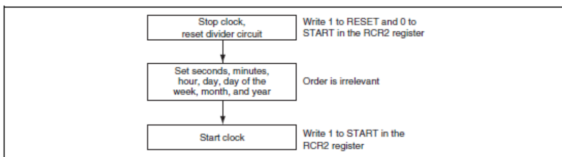
Figure 15.2 Setting Time
