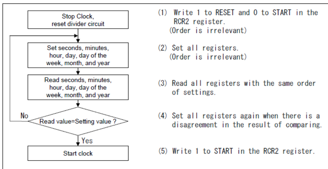
Figure 15.2 Setting Time
