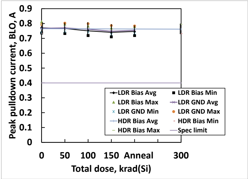
Fig. 24: HS-4080AEH B low side output peak pull-down current as a function of total dose irradiation at low dose rate for the biased (per Figure 1) and unbiased (all pins grounded) cases and at high dose rate for the biased case. The dose rate was 0.01 rad(Si)/s for low dose rate irradiation and 68 rad(Si)/s for high dose rate irradiation. The low dose rate irradiations were followed by a biased anneal at 100°C for 168 hours. Sample sizes were 10 at low dose rate under bias, 10 at low dose rate with all pins grounded and 20 samples at high dose rate under bias. The SMD post-irradiation specification limit is 400.0mA minimum. The B high side, A low side and A high side pull-down current responses (not shown) were closely similar. (135)
