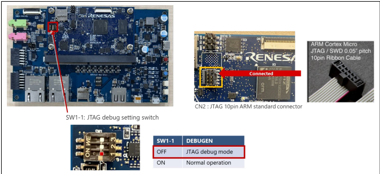
Figure 22: JTAG connection
