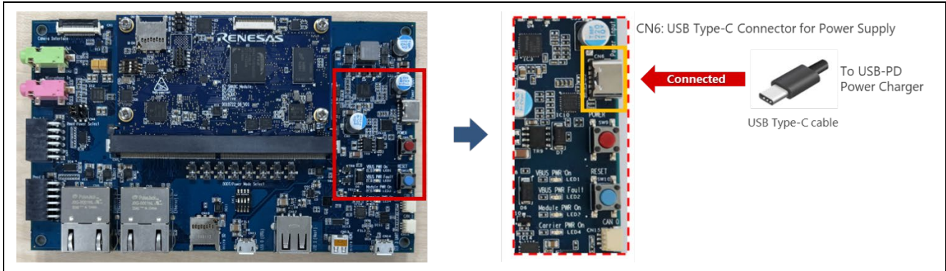
Figure 24: Power Supply
