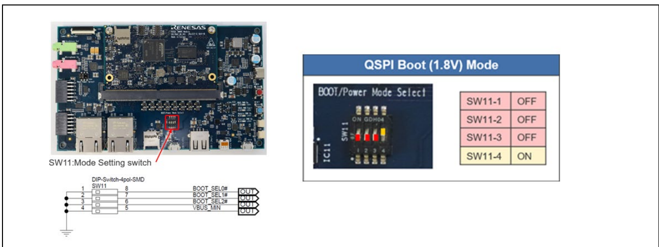
Figure 21: Boot MODE
