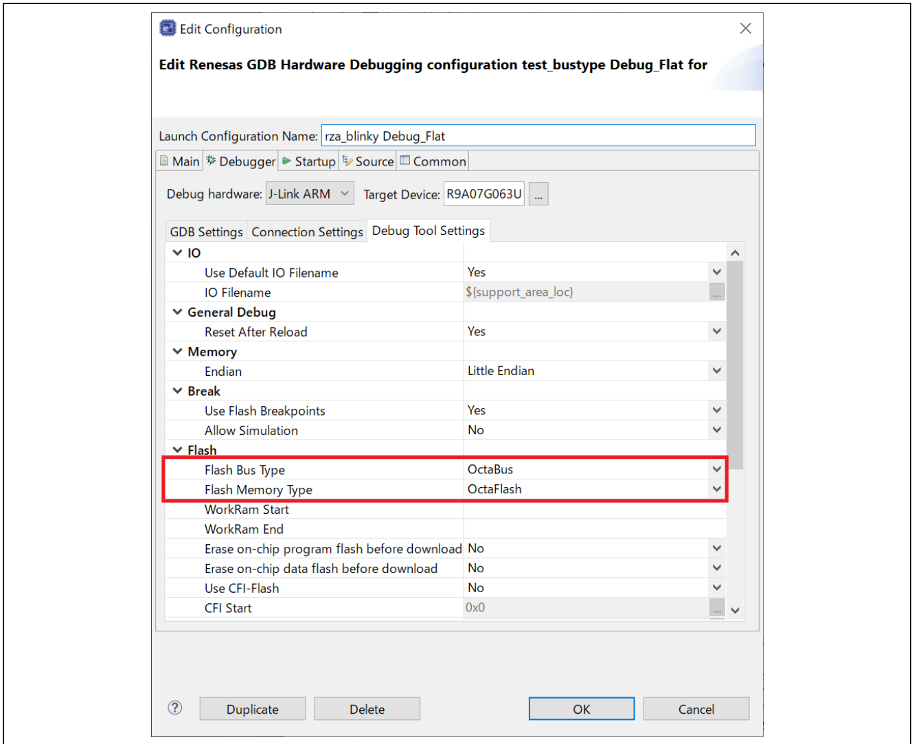
Figure 95 : Flash related settings in Debug Tool Settings
