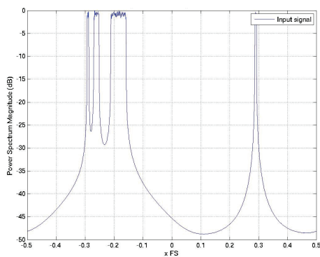
INPUT SIGNAL SPECTRUM
