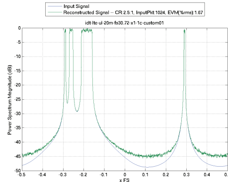
OUTPUT SIGNAL SPECTRUM
