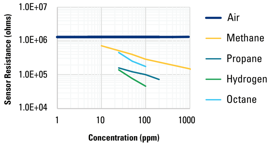
SGAS711 RESPONSE
