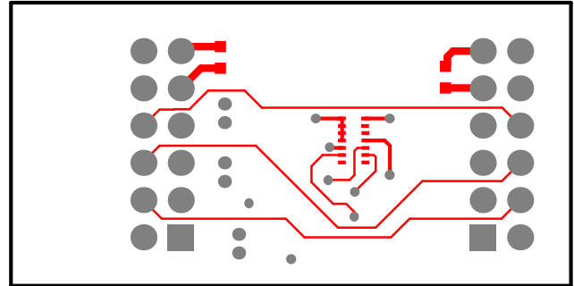
Figure 6. Copper Top
