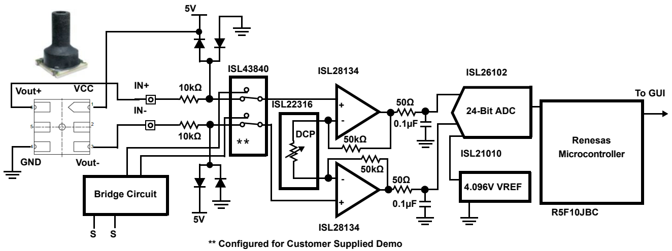
Figure 2. Simplified Pressure Gauge Schematic
