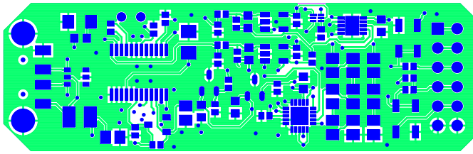
Figure 12. Top Layer
