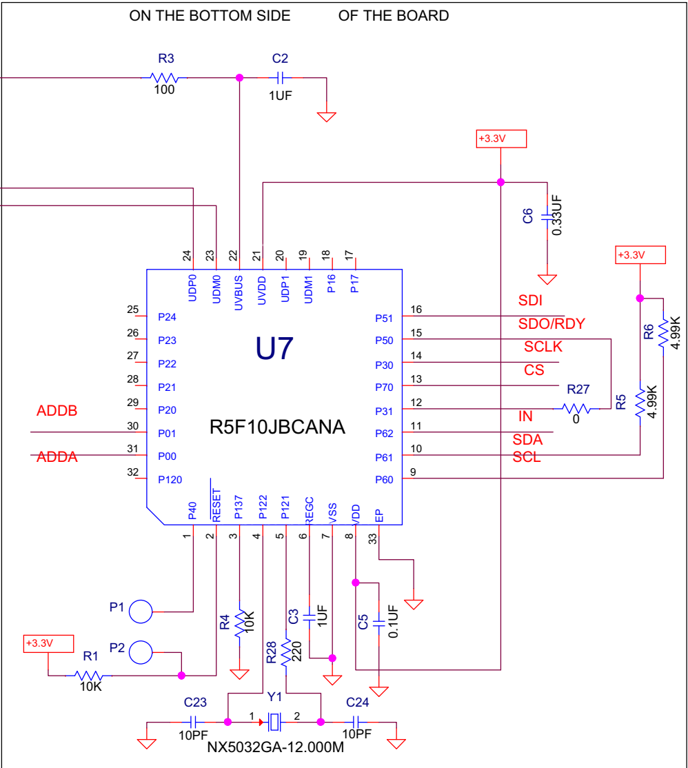
Figure 20. RTKA-BDGSTKEV2Z MCU Schematic
