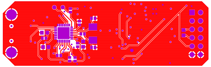
Figure 13. Bottom Layer
