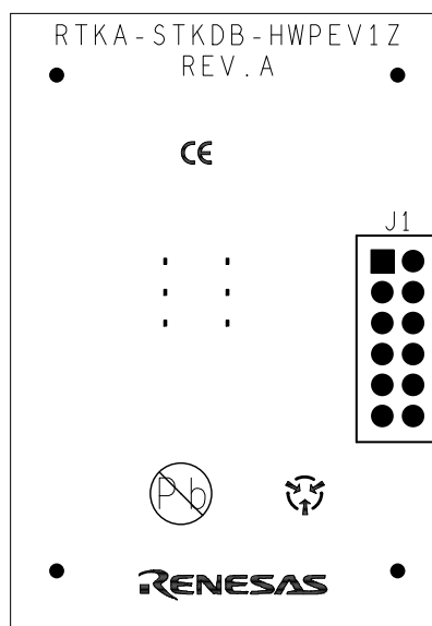
Figure 18. Assembly Drawing
