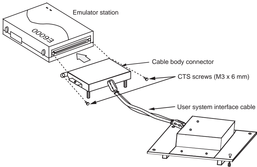
Figure 2 Connecting User System Interface Cable to Emulator Station
