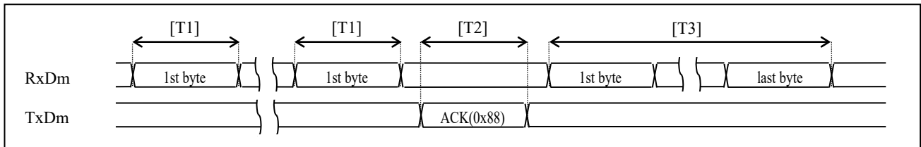
Figure 5-15 Transmit timing chart (APP MCU) (Timeout occurs)
