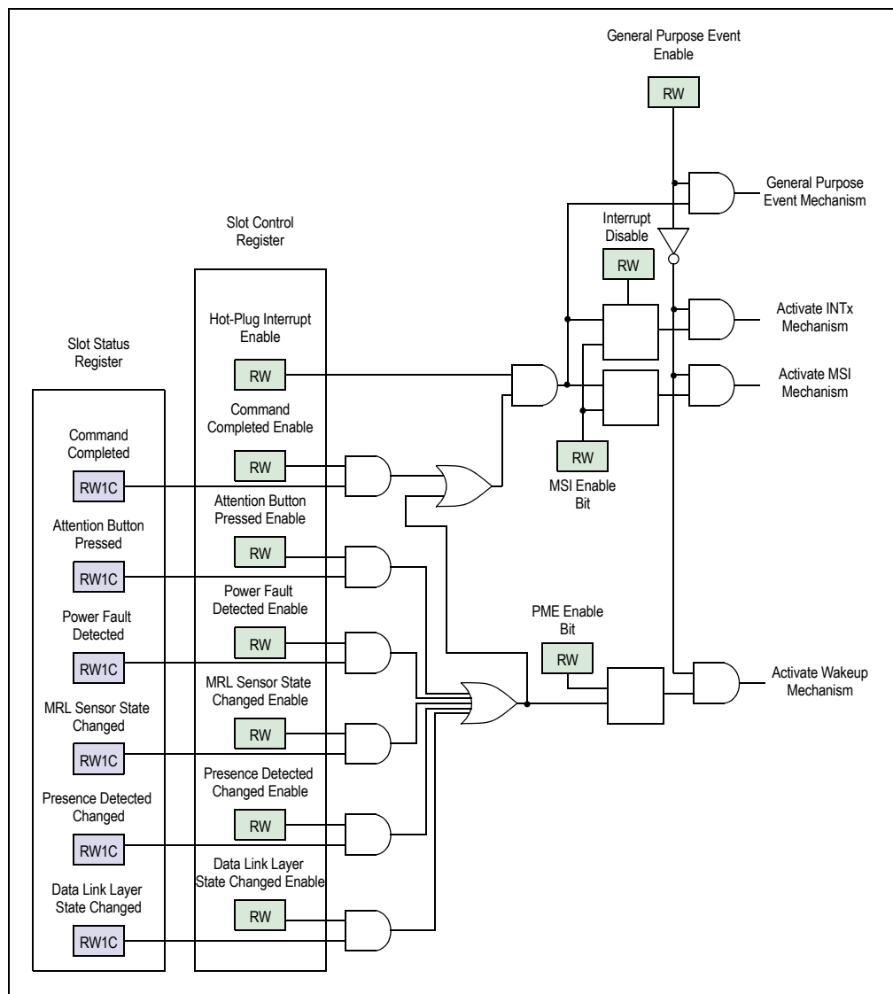
Figure 7.4 PES16T4AG2 Hot-Plug Event Signalling
