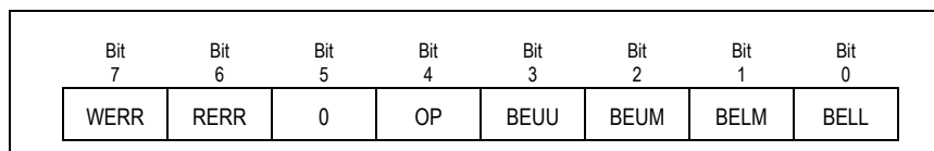
Figure 5.6 CSR Register Read or Write CMD Field Format
