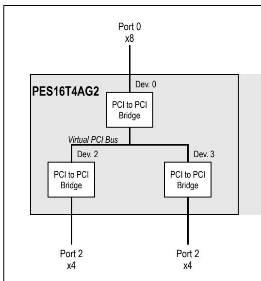
Figure 1.4 Two Ports Merged Configuration
