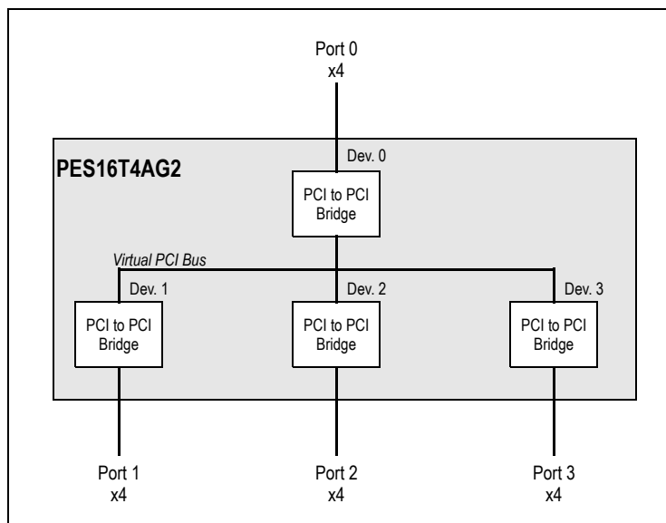
Figure 1.3 All Ports Unmerged Configuration
