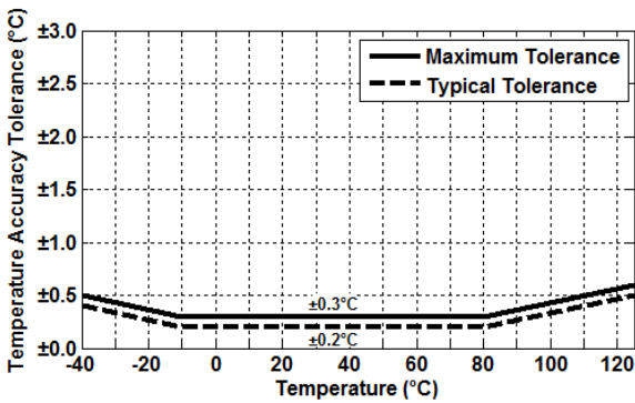
Figure 10. HS3101/HS3102 Temperature Sensor Accuracy Tolerance
