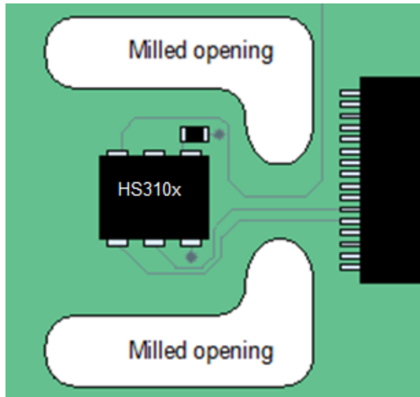
Figure 20. Milled PCB Openings for Thermal Isolation
