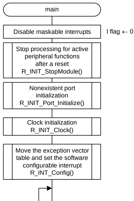
Figure 5.3 Main Processing
