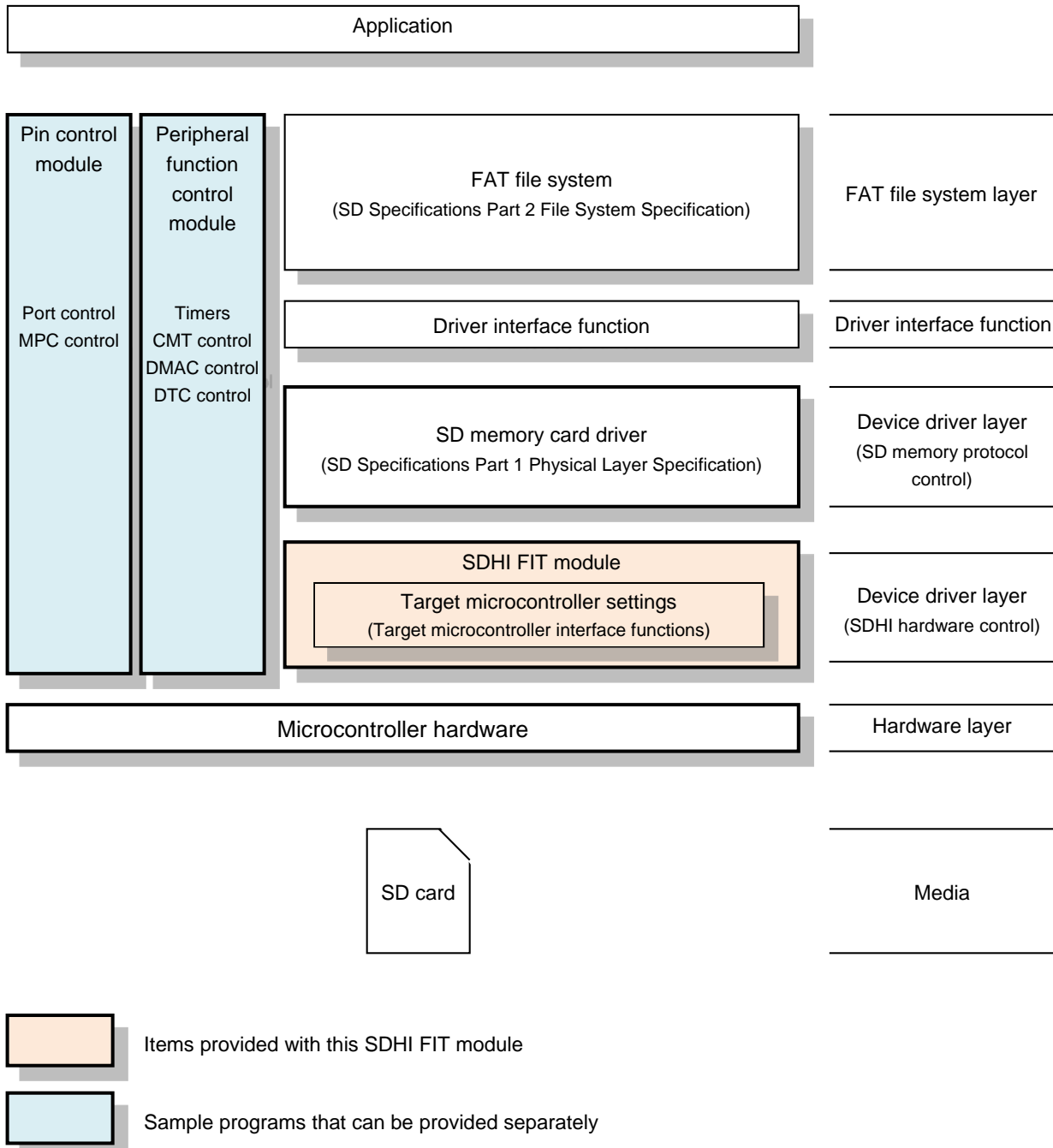
Figure 1.1 Application Structure
