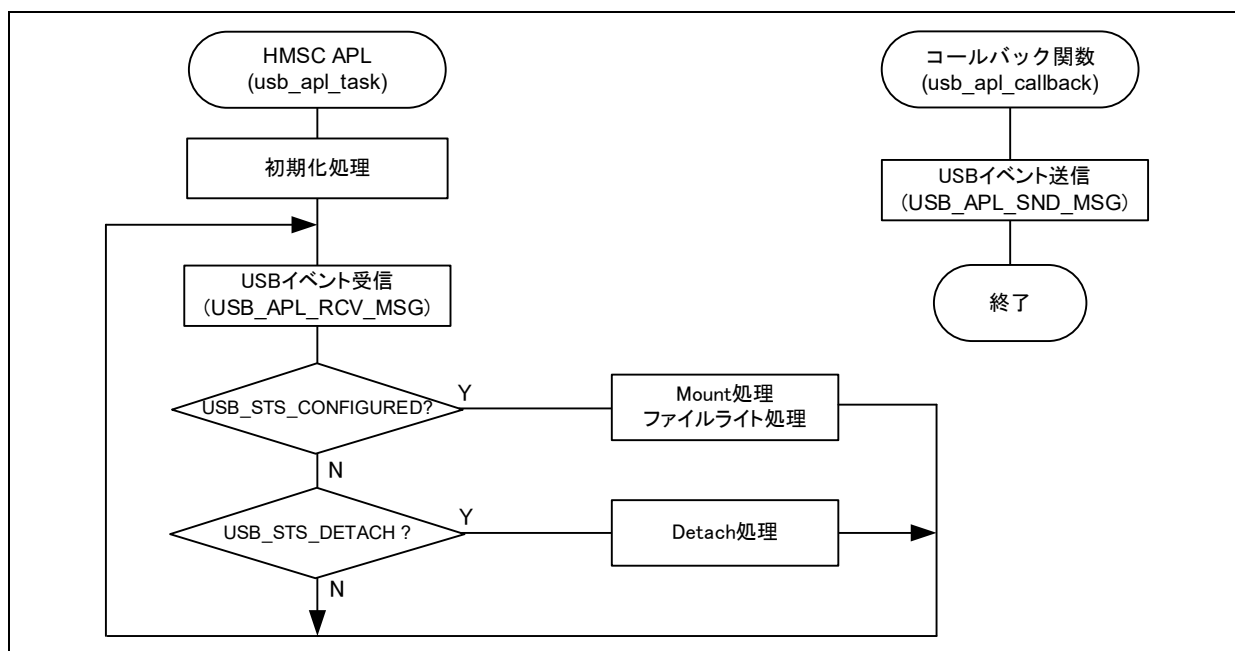
Figure 4-2 usb_apl_task
