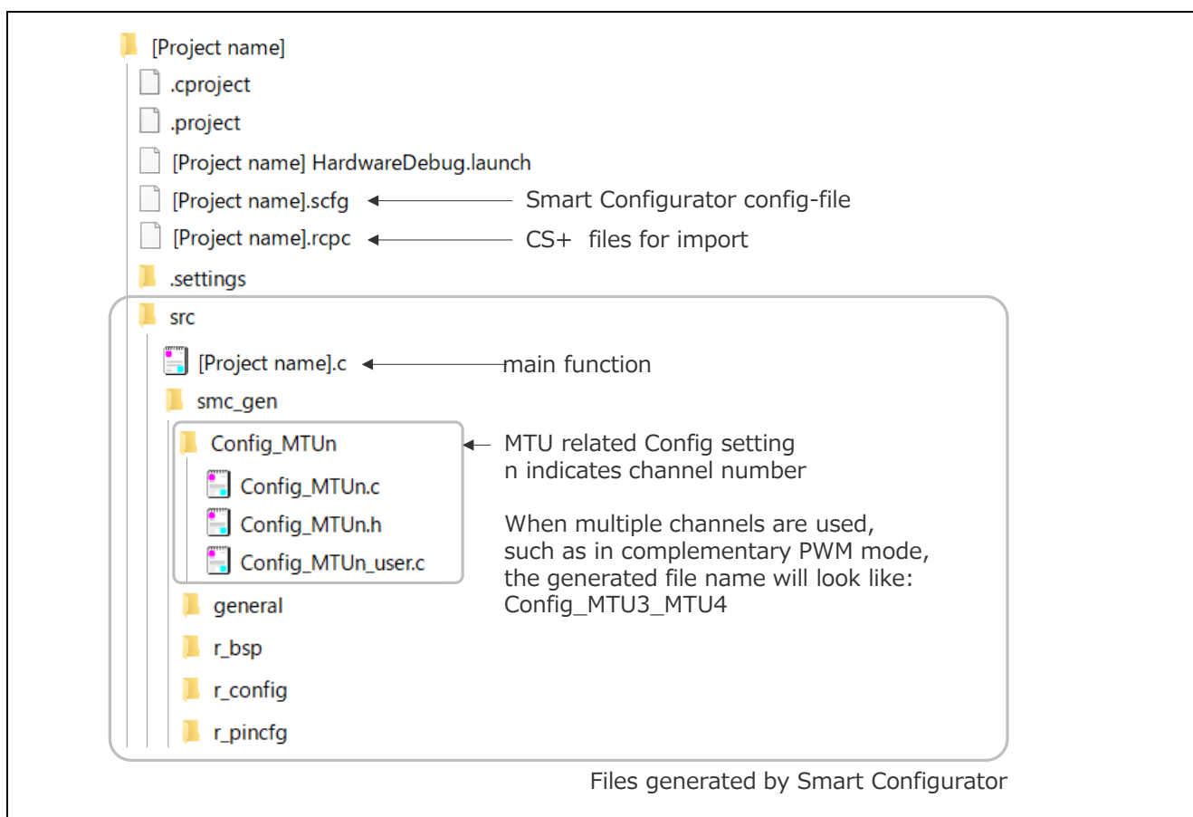
Figure 3.1 MTU Folder Structure
