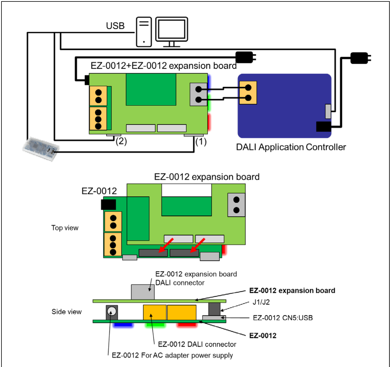
Figure 4-3 Connection diagram when using EZ-0012 expansion board
