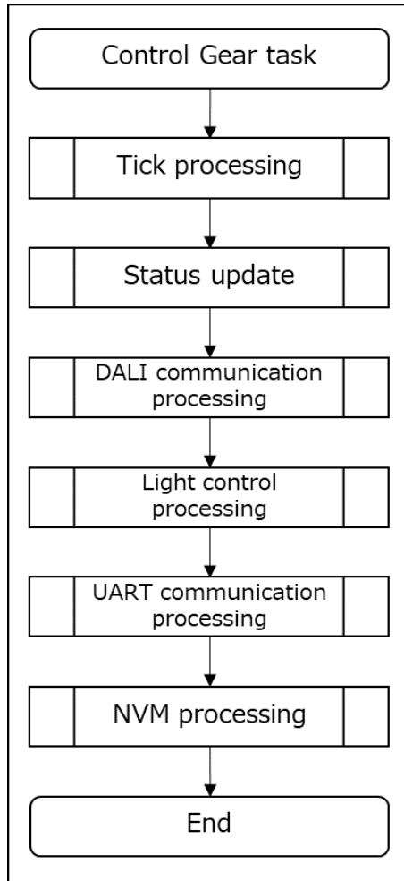
Figure 4-17 Control Gear task processing flow diagram
