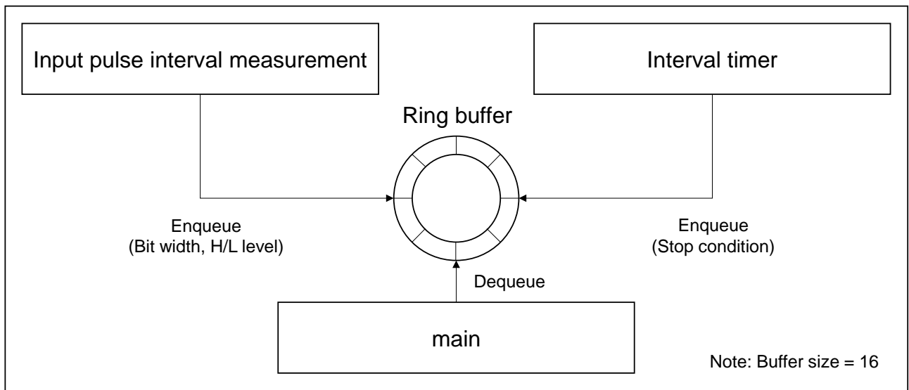
Figure 5-1 Receiver (Rx) overview
