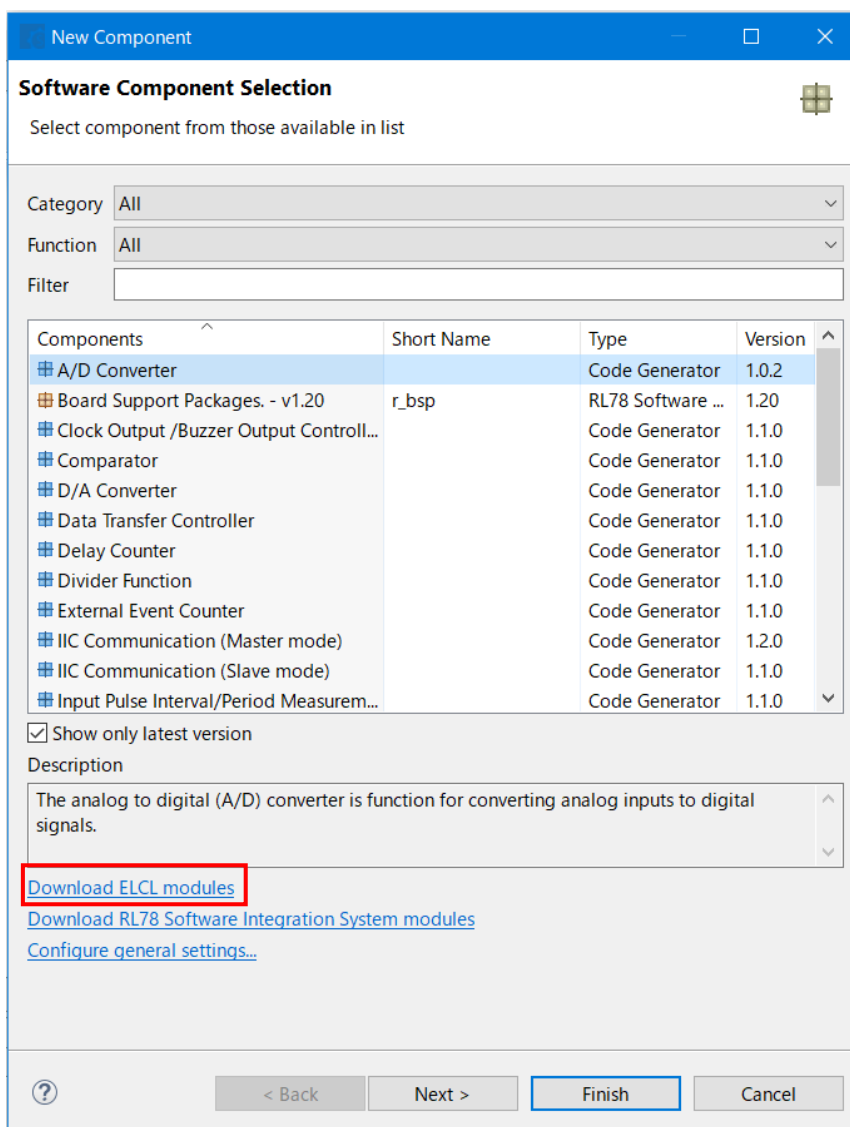
Figure 4-31 Add component
