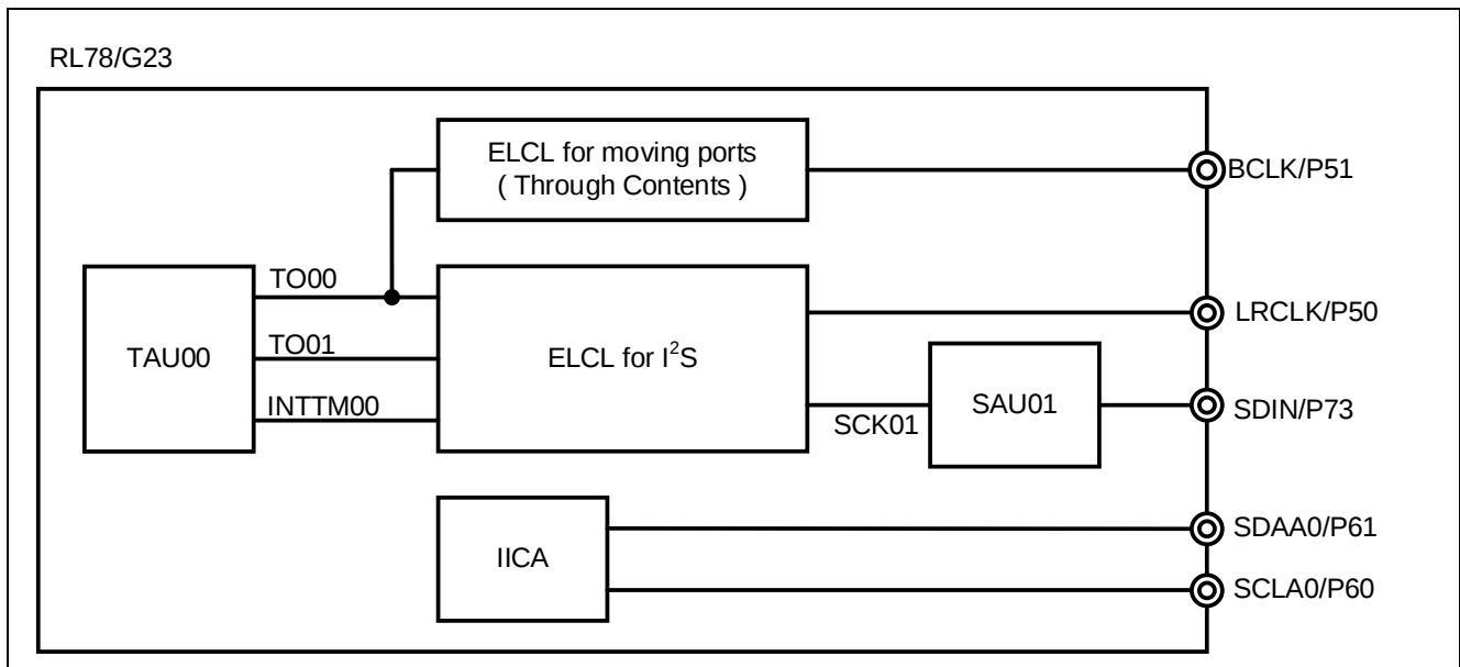
Figure 4-1 System configuration of the sample code
