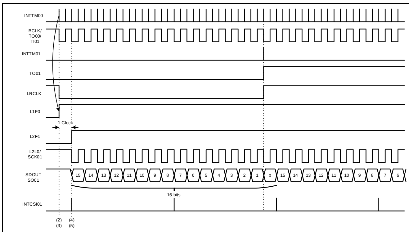
Figure 1-3 Timing chart of I 2 S communication (master) using ELCL
