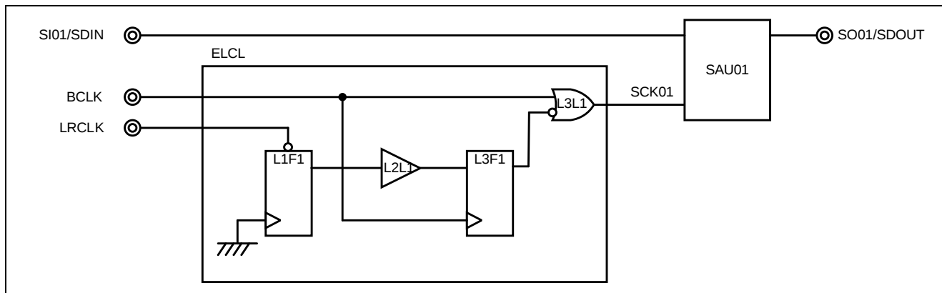
Figure 1-4 System Configuration of I 2 S communication (slave) using ELCL
