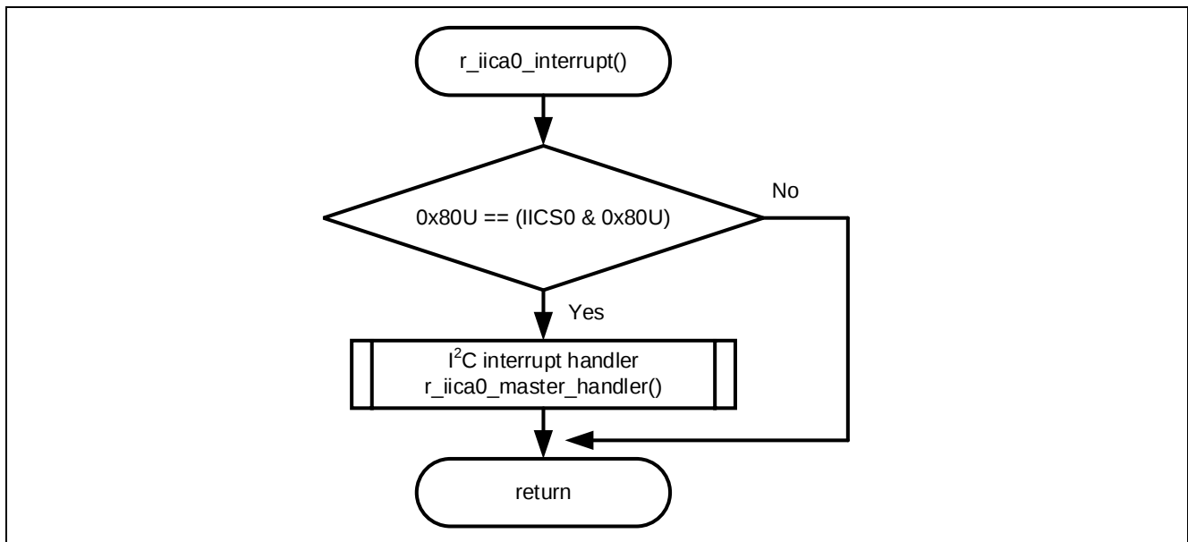
Figure 4-23 IICA0 interrupt process
