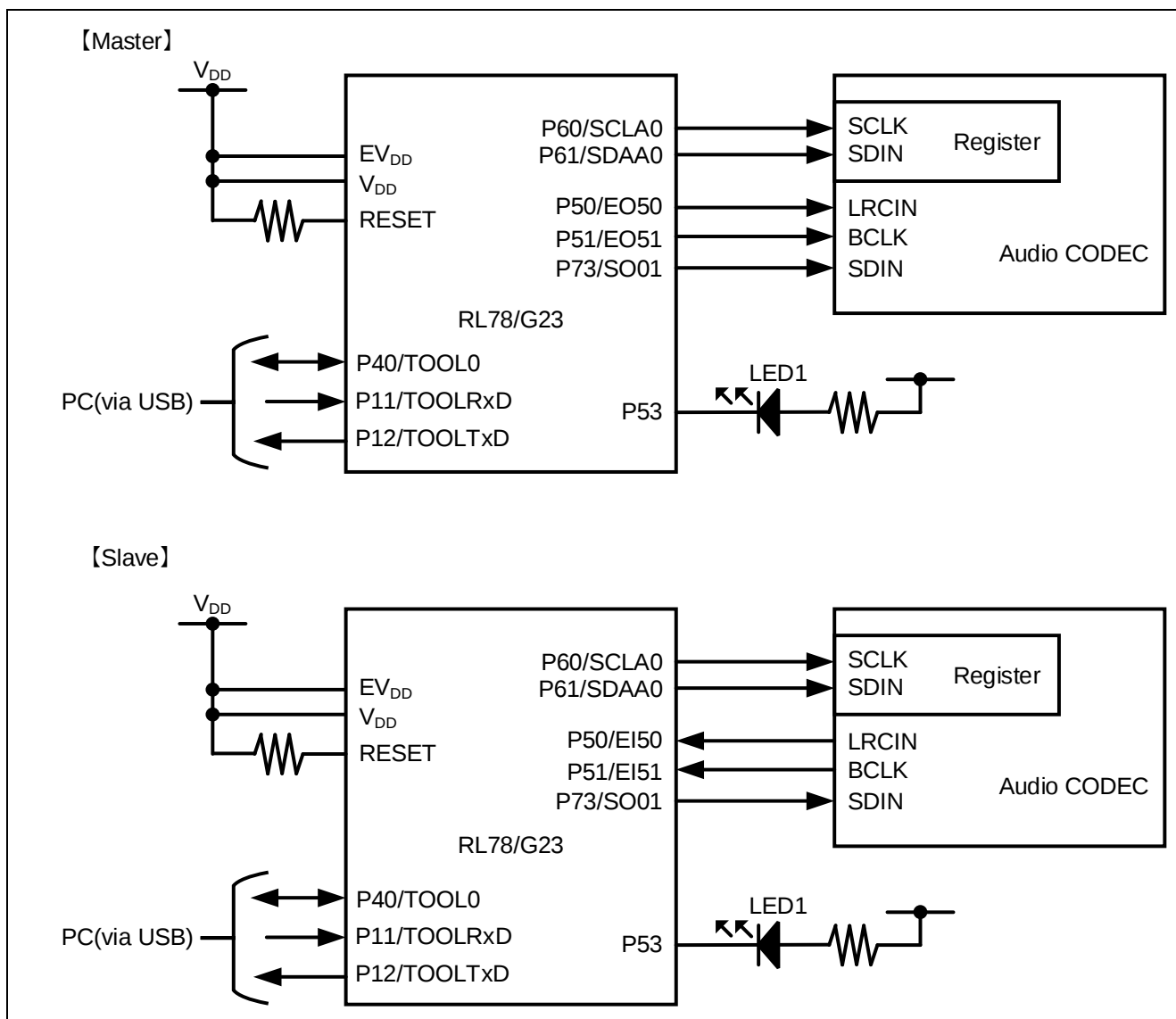
Figure 3-1 Hardware Configuration
