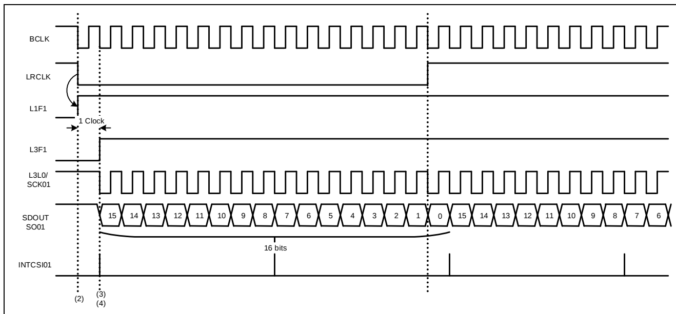
Figure 1-5 Timing chart of I 2 S communication (slave) using ELCL
