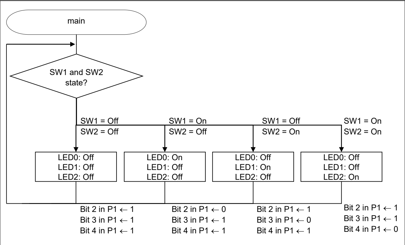
Figure 4.5 Main Processing
