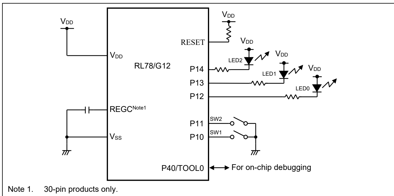
Figure 3.1 Hardware Configuration
