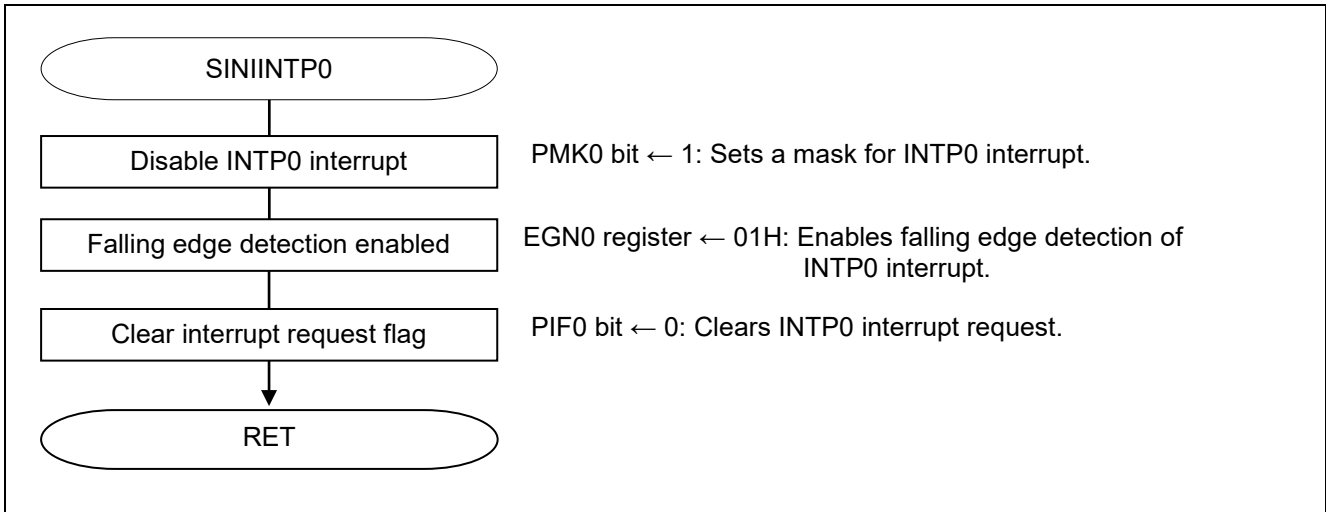
Figure 5.9 Interrupt Setup
