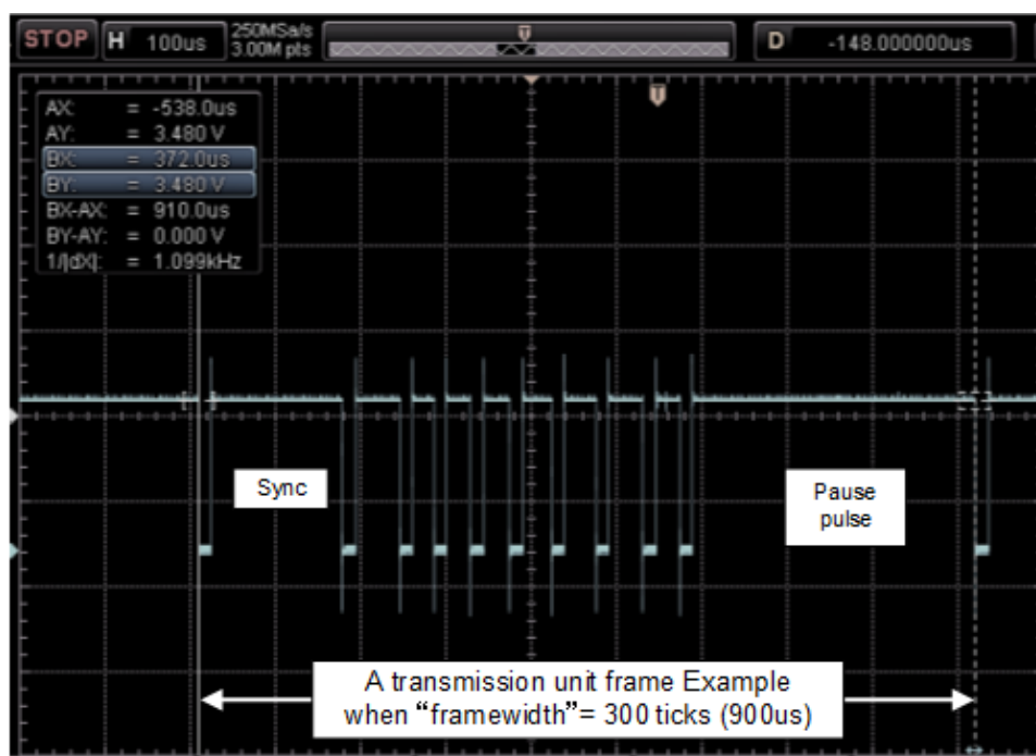
Figure 1-2 Real SENT Waveforms Generated by this Example
