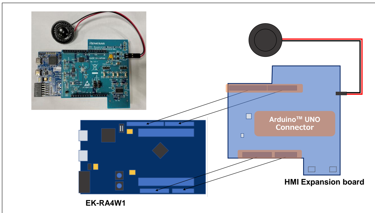
Figure 2.1 Board connection
