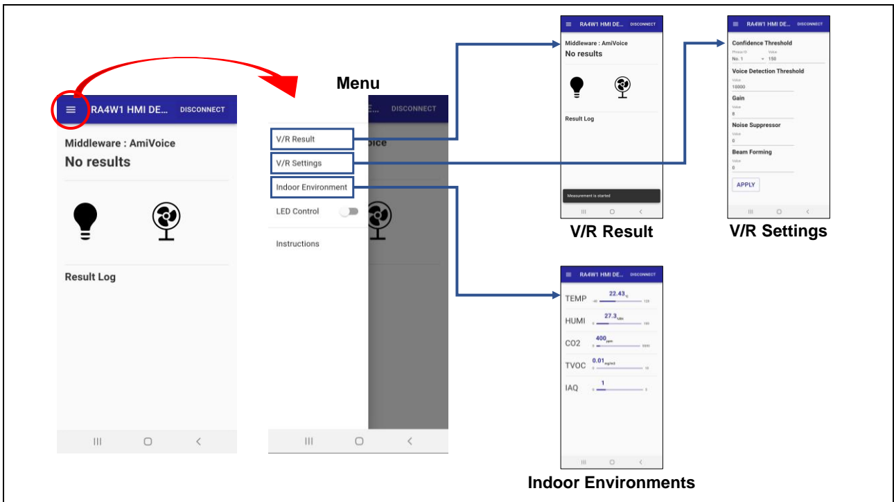
Figure 3.2 Screen Transition
