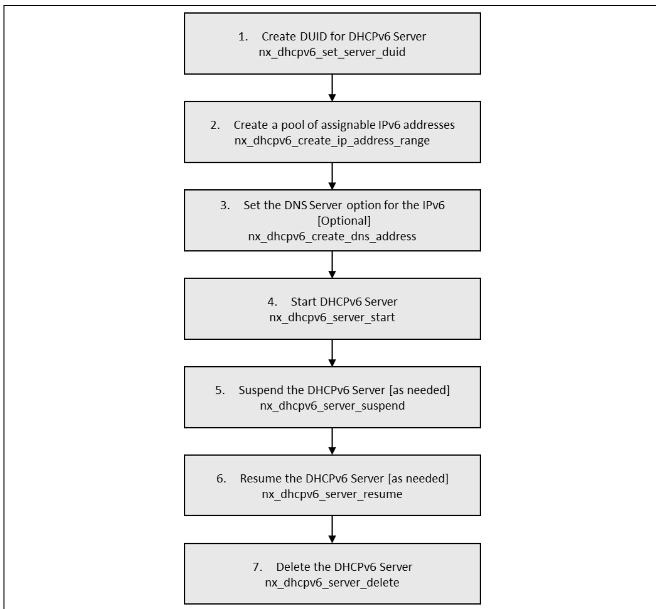
Figure 3. Flow Diagram of a Typical NetX Duo DHCPv6 Server Module Application
