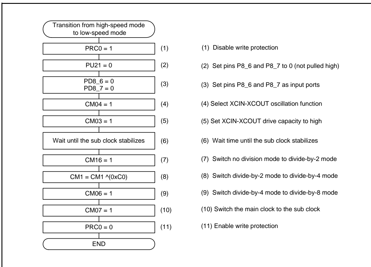
Figure 3.2 Transition Procedure from High-Speed Mode to Low-Speed Mode
