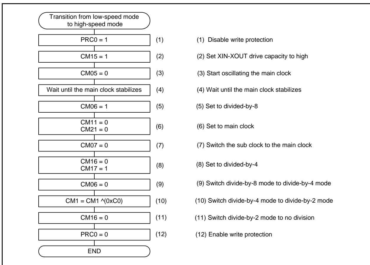
Figure 3.5 Transition Procedure from Low-Speed Mode to High-Speed Mode
