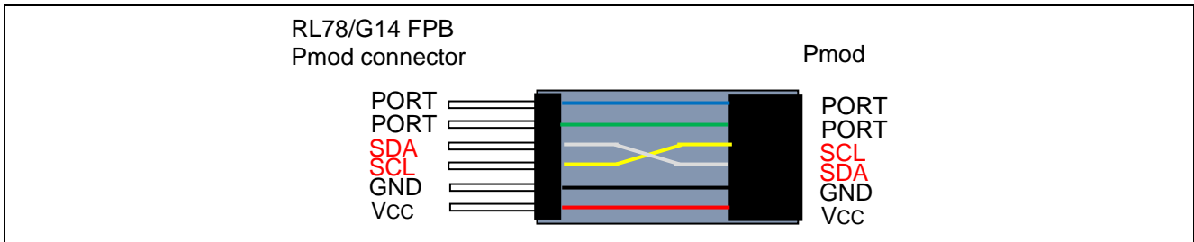
Figure 1.1 Signal conversion
