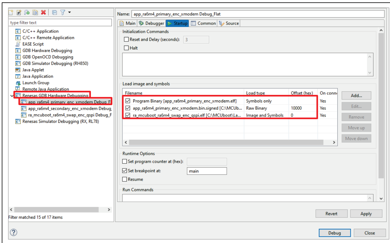
Figure 11. Debug Configurations
