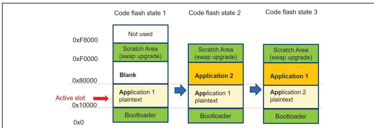
Figure 5. Operational Flow with Swap Update Mode
