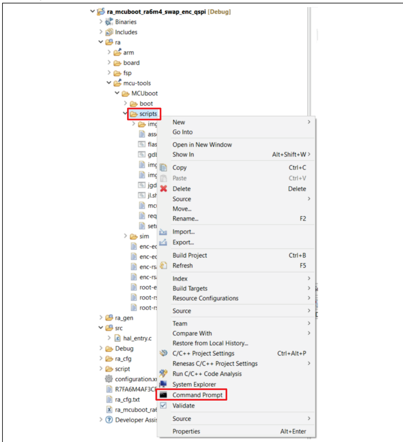
Figure 53. Start Command Prompt under the \MCUboot\scripts Folder
