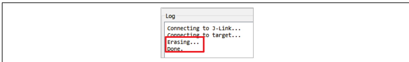
Figure 8. Erase Successful
