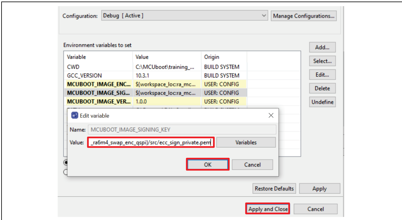
Figure 57. Configure the Application Project to use the Custom Image Signing
