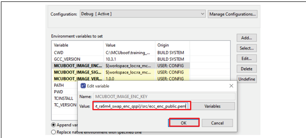
Figure 58. Configure the Application Project to use the Custom Key for the Image Encryption Process
