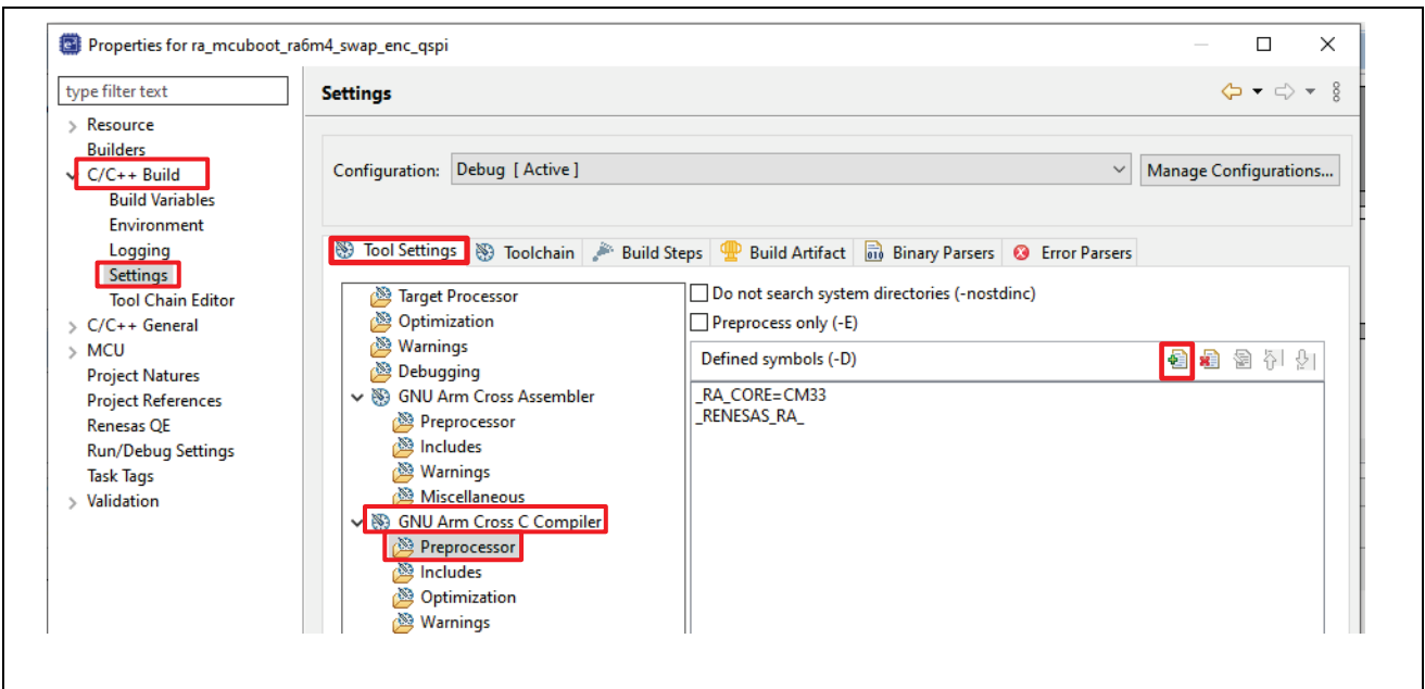
Figure 25. Add Preprocessor Setting
