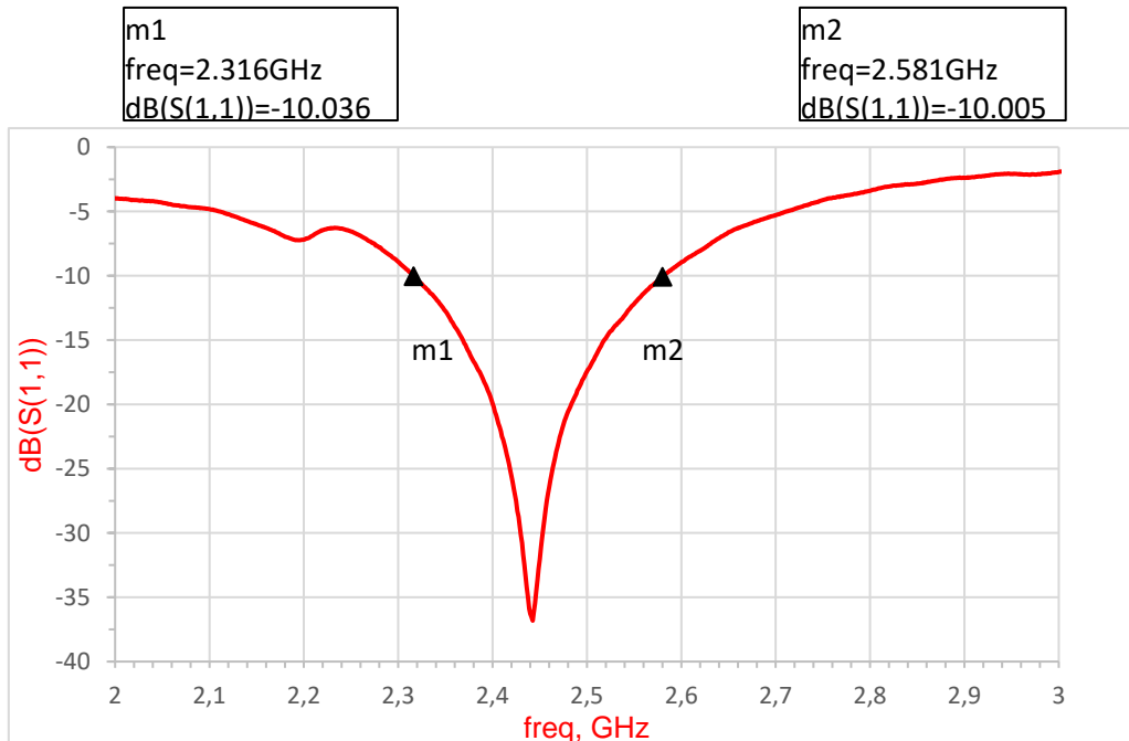
Figure 25. Measured S11, ZOR antenna, 1.0 mm substrate
