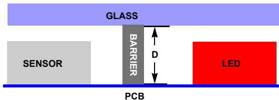
FIGURE 12. DIAGRAM OF PROXIMITY SET-UP HIGHLIGHTING THE HEIGHT OF THE BARRIER
