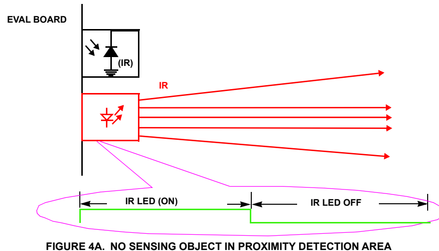
FIGURE 4A. NO SENSING OBJECT IN PROXIMITY DETECTION AREA
