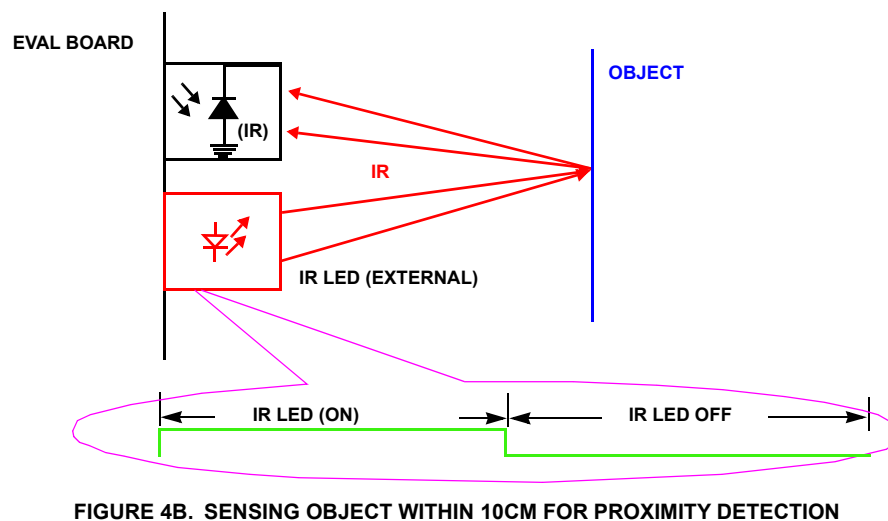
FIGURE 4B. SENSING OBJECT WITHIN 10CM FOR PROXIMITY DETECTION
